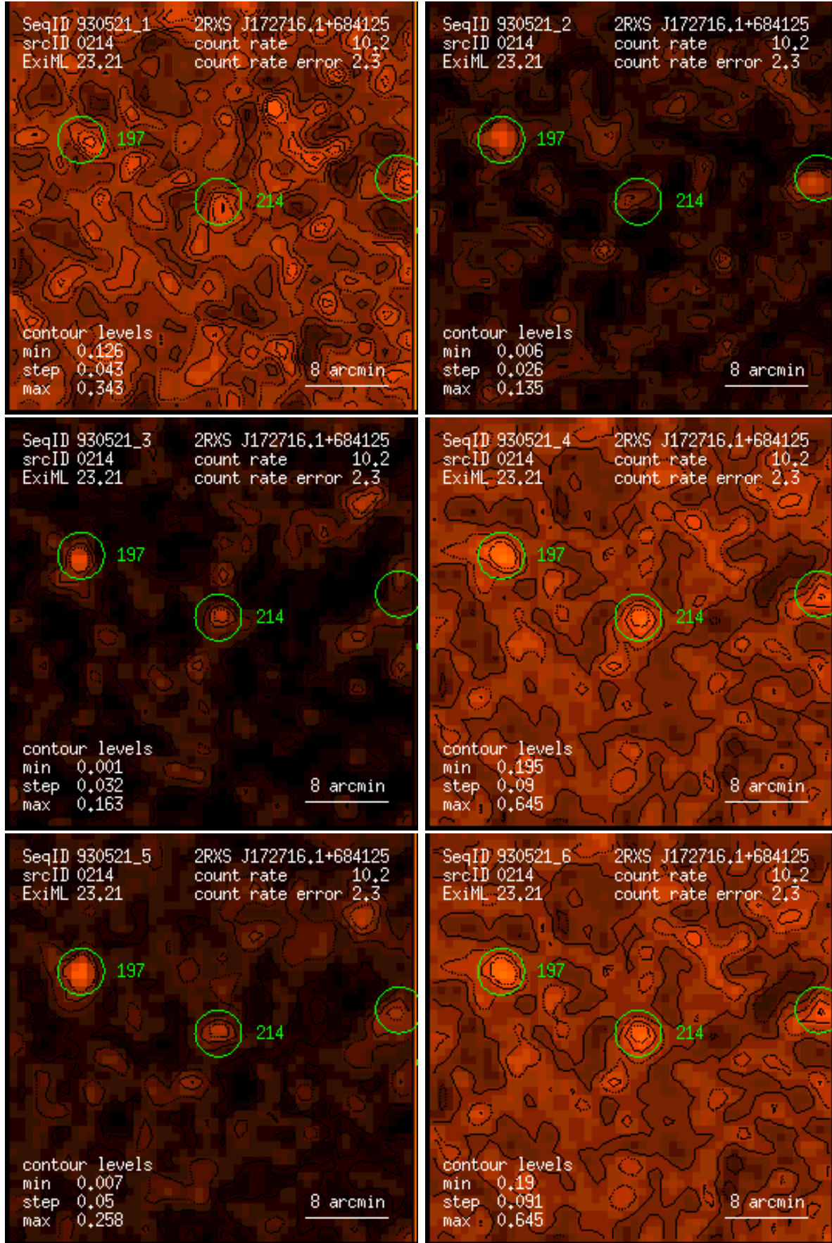
Figure 214: RASS 930521: detection 0214: band rate images, Gaussian filter: (1) PSPC channels 11 – 41, (2) 52 – 90, (3) 91 – 201, (4) 11 – 235, (5) 52 – 201, (6) 11 – 201. Broad band rates in counts/ks. Band rate contour levels in counts/ks/arcmin 2 .
