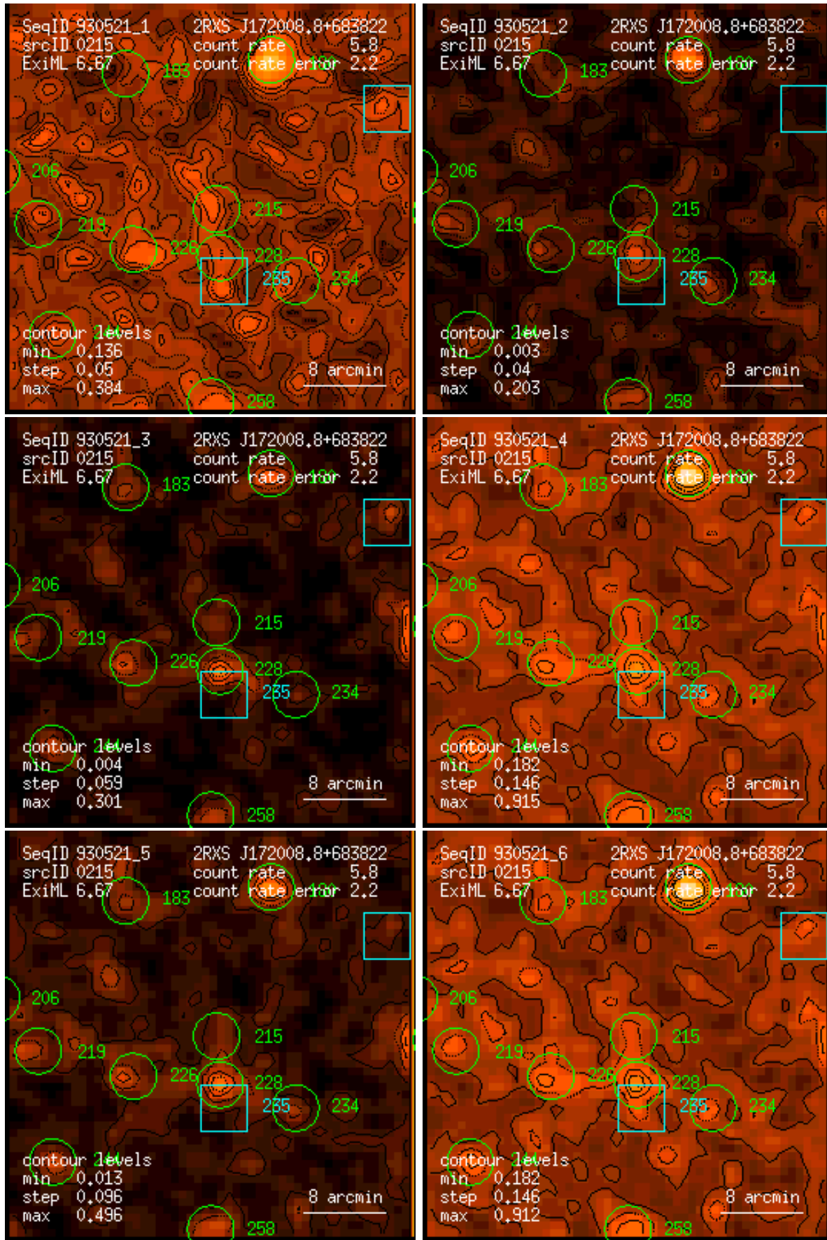
Figure 215: RASS 930521: detection 0215: band rate images, Gaussian filter: (1) PSPC channels 11 – 41, (2) 52 – 90, (3) 91 – 201, (4) 11 – 235, (5) 52 – 201, (6) 11 – 201. Broad band rates in counts/ks. Band rate contour levels in counts/ks/arcmin 2 .
