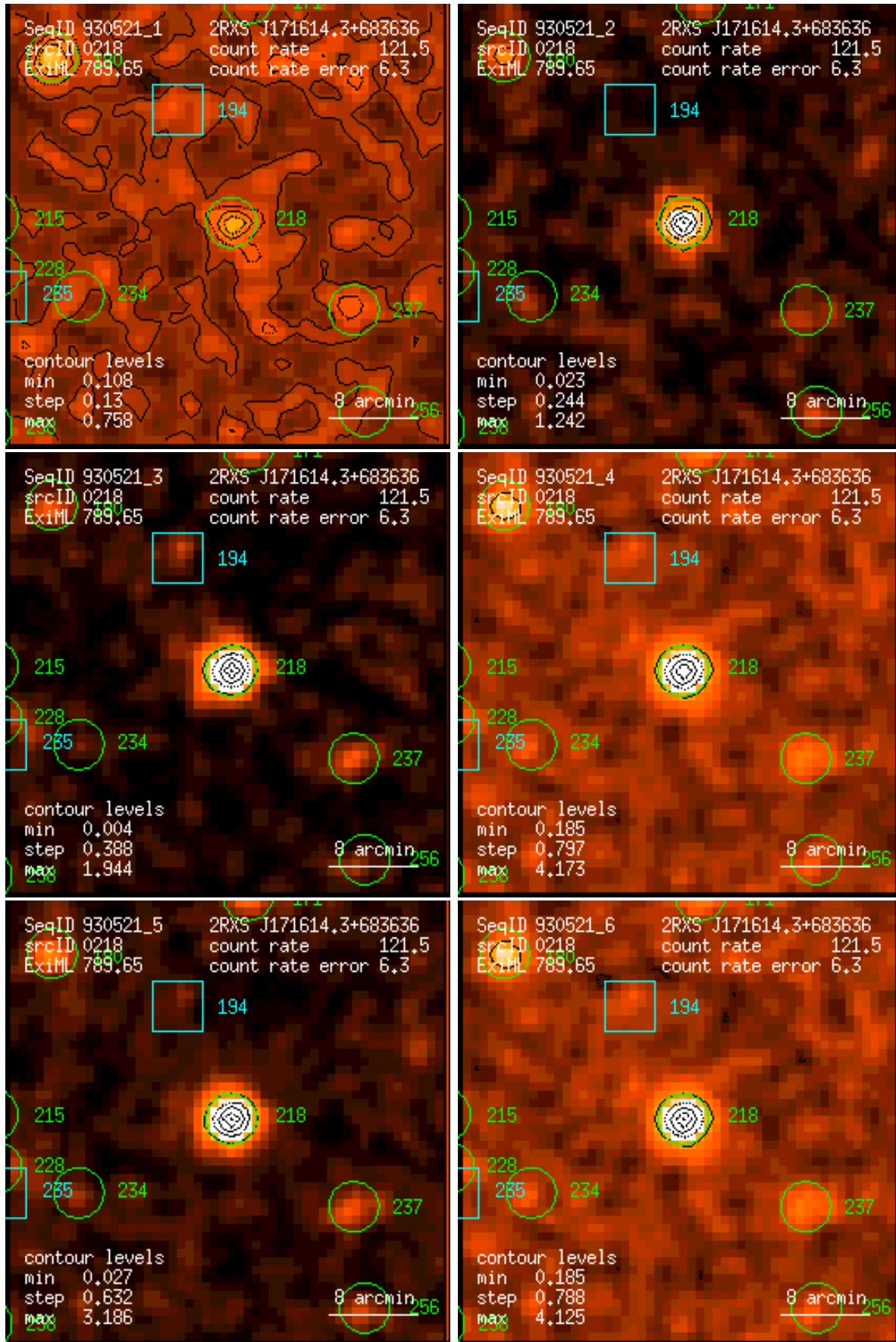
Figure 218: RASS 930521: detection 0218: band rate images, Gaussian filter: (1) PSPC channels 11 – 41, (2) 52 – 90, (3) 91 – 201, (4) 11 – 235, (5) 52 – 201, (6) 11 – 201. Broad band rates in counts/ks. Band rate contour levels in counts/ks/arcmin 2 .
