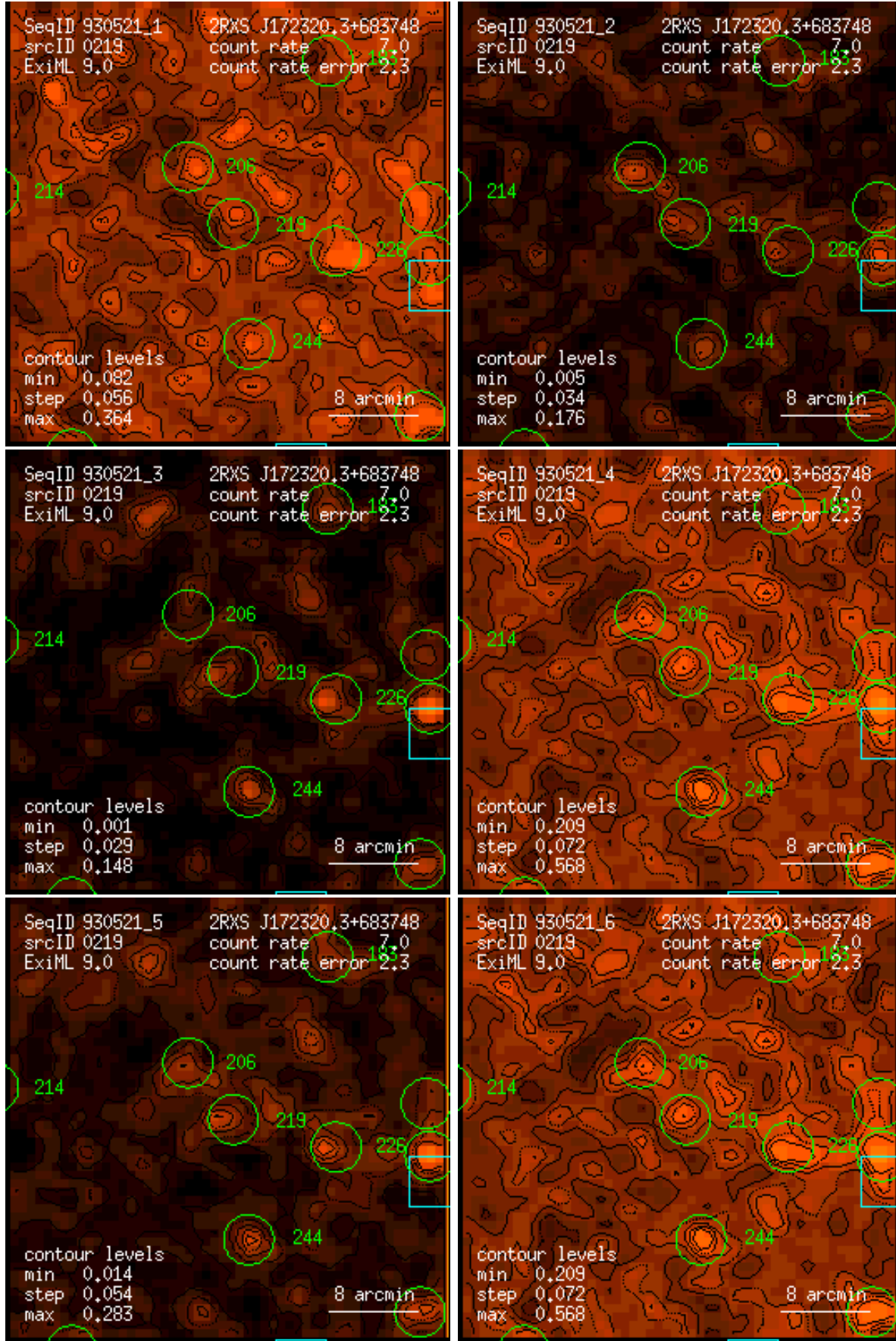
Figure 219: RASS 930521: detection 0219: band rate images, Gaussian filter: (1) PSPC channels 11 – 41, (2) 52 – 90, (3) 91 – 201, (4) 11 – 235, (5) 52 – 201, (6) 11 – 201. Broad band rates in counts/ks. Band rate contour levels in counts/ks/arcmin 2 .
