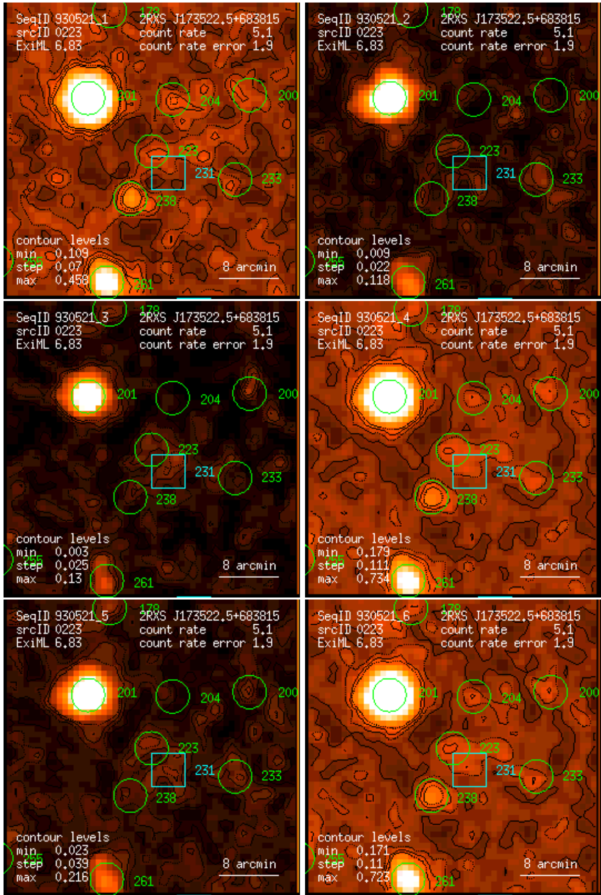
Figure 223: RASS 930521: detection 0223: band rate images, Gaussian filter: (1) PSPC channels 11 – 41, (2) 52 – 90, (3) 91 – 201, (4) 11 – 235, (5) 52 – 201, (6) 11 – 201. Broad band rates in counts/ks. Band rate contour levels in counts/ks/arcmin 2 .
