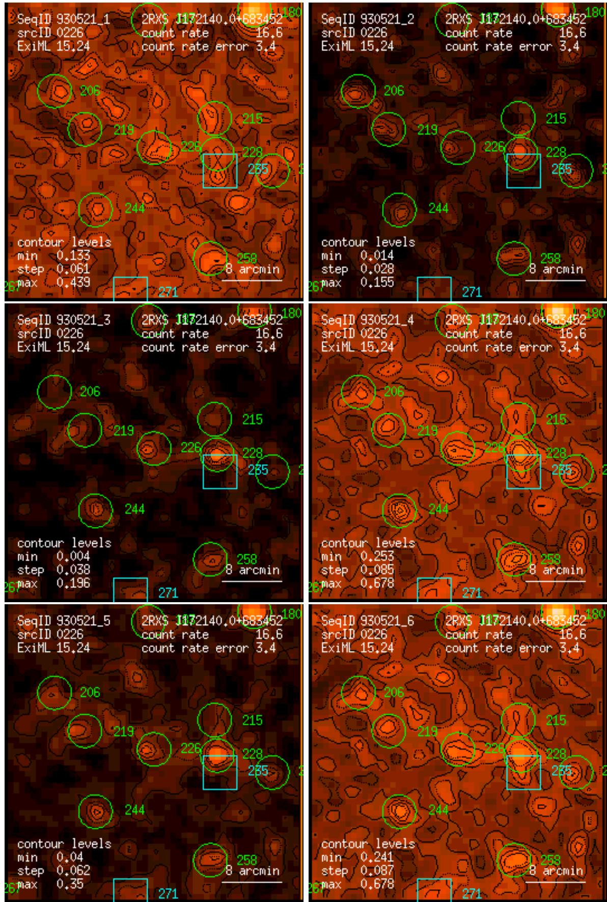
Figure 226: RASS 930521: detection 0226: band rate images, Gaussian filter: (1) PSPC channels 11 – 41, (2) 52 – 90, (3) 91 – 201, (4) 11 – 235, (5) 52 – 201, (6) 11 – 201. Broad band rates in counts/ks. Band rate contour levels in counts/ks/arcmin 2 .
