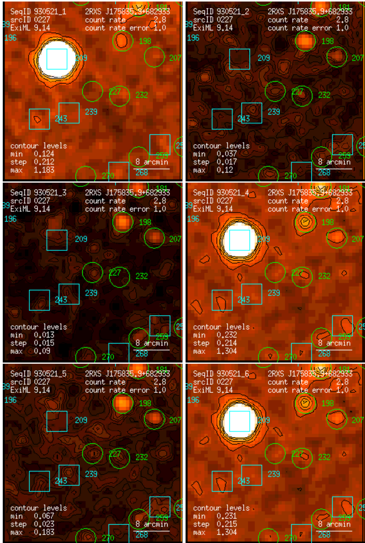
Figure 227: RASS 930521: detection 0227: band rate images, Gaussian filter: (1) PSPC channels 11 – 41, (2) 52 – 90, (3) 91 – 201, (4) 11 – 235, (5) 52 – 201, (6) 11 – 201. Broad band rates in counts/ks. Band rate contour levels in counts/ks/arcmin 2 .
