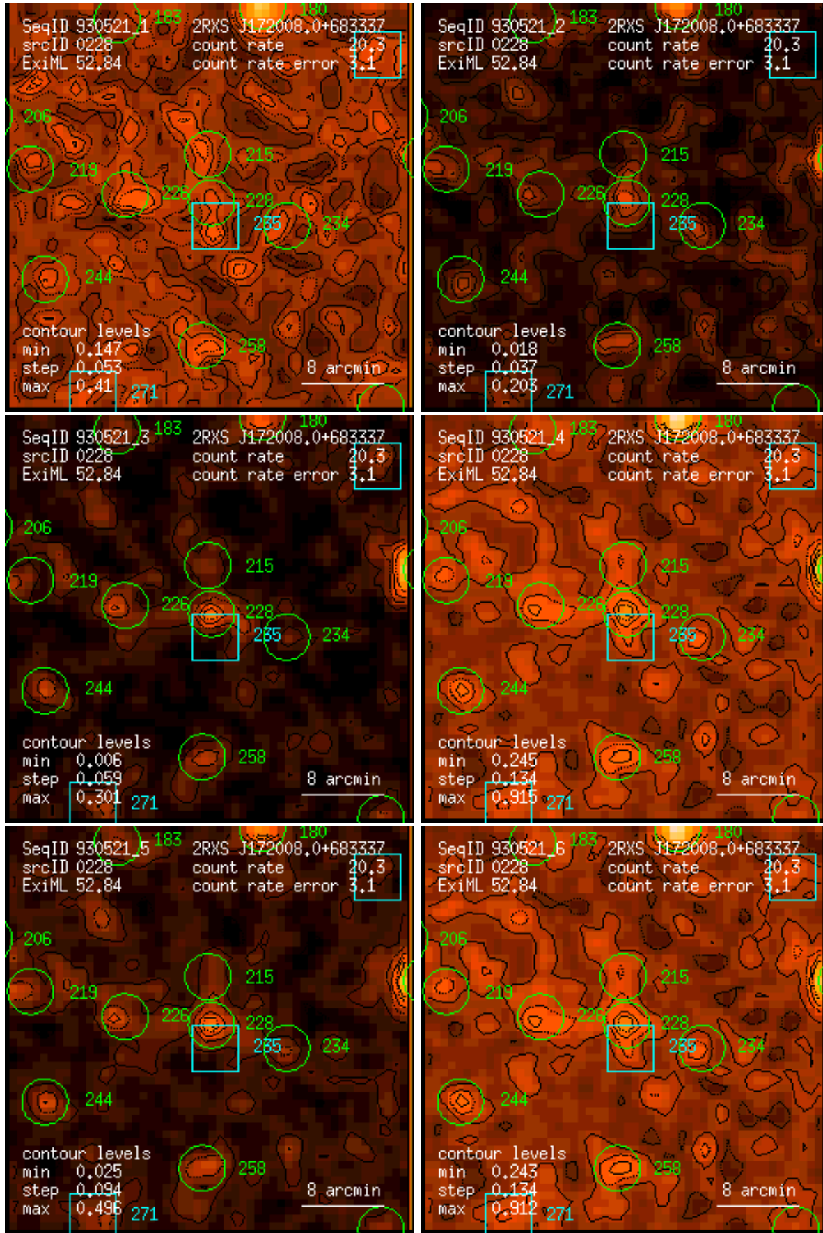
Figure 228: RASS 930521: detection 0228: band rate images, Gaussian filter: (1) PSPC channels 11 – 41, (2) 52 – 90, (3) 91 – 201, (4) 11 – 235, (5) 52 – 201, (6) 11 – 201. Broad band rates in counts/ks. Band rate contour levels in counts/ks/arcmin 2 .
