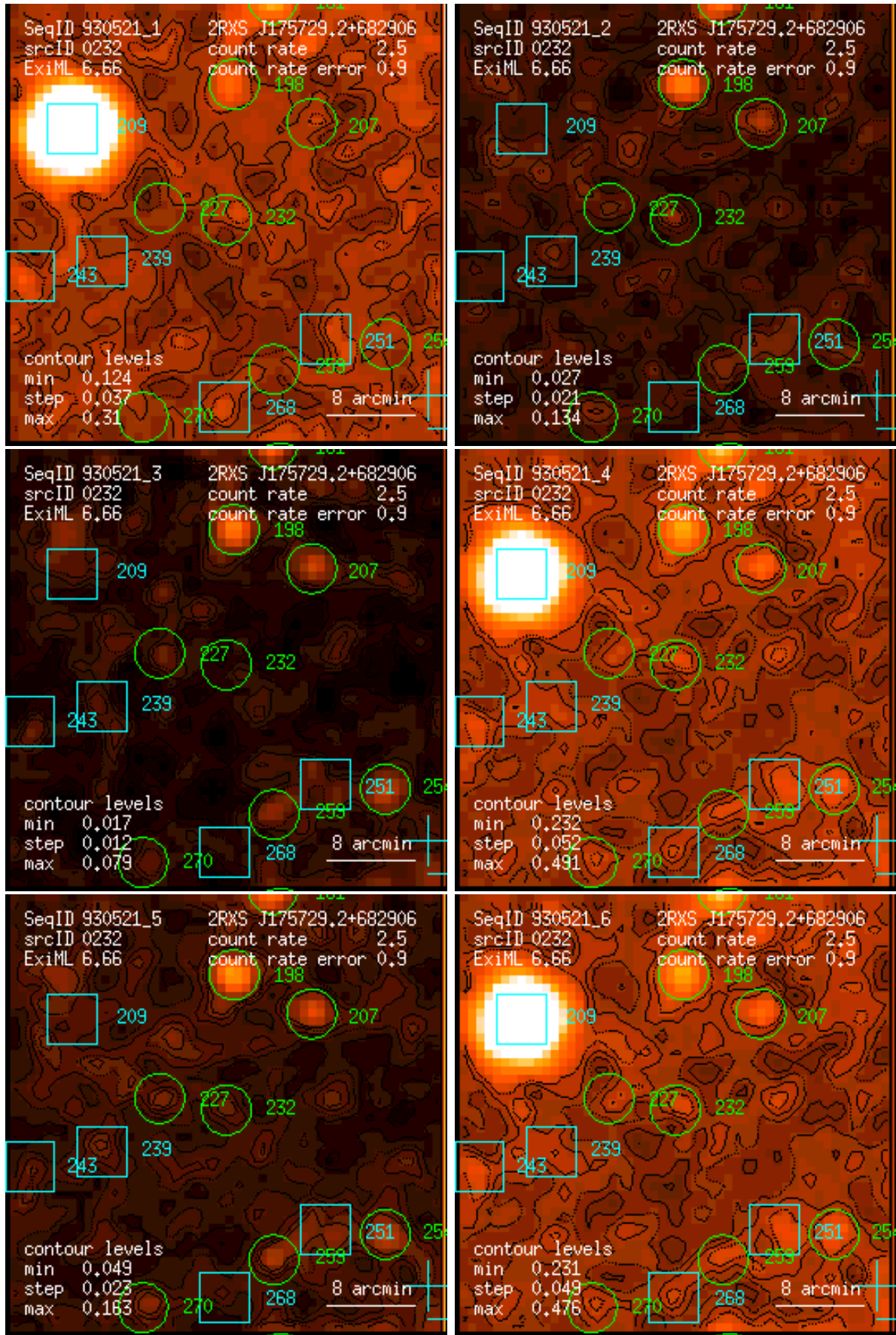
Figure 232: RASS 930521: detection 0232: band rate images, Gaussian filter: (1) PSPC channels 11 – 41, (2) 52 – 90, (3) 91 – 201, (4) 11 – 235, (5) 52 – 201, (6) 11 – 201. Broad band rates in counts/ks. Band rate contour levels in counts/ks/arcmin 2 .
