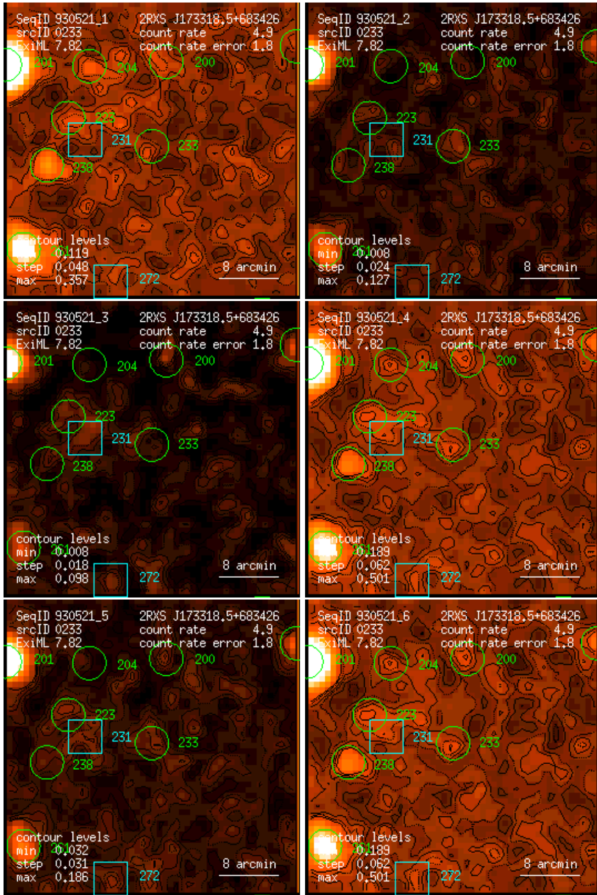
Figure 233: RASS 930521: detection 0233: band rate images, Gaussian filter: (1) PSPC channels 11 – 41, (2) 52 – 90, (3) 91 – 201, (4) 11 – 235, (5) 52 – 201, (6) 11 – 201. Broad band rates in counts/ks. Band rate contour levels in counts/ks/arcmin 2 .
