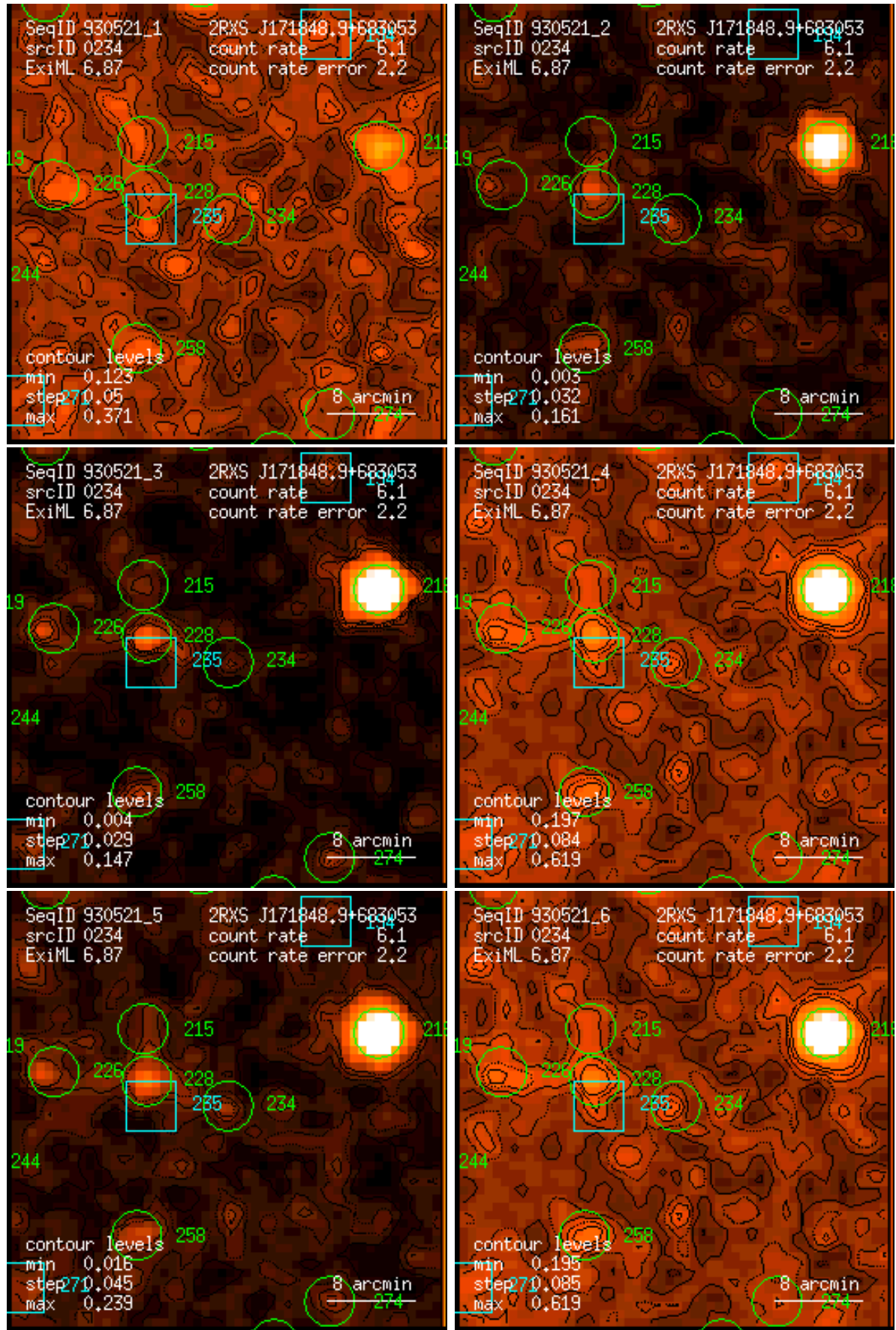
Figure 234: RASS 930521: detection 0234: band rate images, Gaussian filter: (1) PSPC channels 11 – 41, (2) 52 – 90, (3) 91 – 201, (4) 11 – 235, (5) 52 – 201, (6) 11 – 201. Broad band rates in counts/ks. Band rate contour levels in counts/ks/arcmin 2 .
