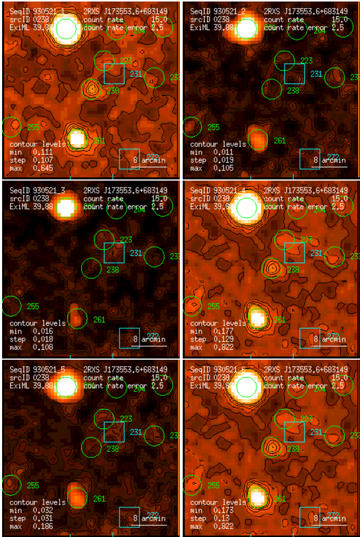
Figure 238: RASS 930521: detection 0238: band rate images, Gaussian filter: (1) PSPC channels 11 – 41, (2) 52 – 90, (3) 91 – 201, (4) 11 – 235, (5) 52 – 201, (6) 11 – 201. Broad band rates in counts/ks. Band rate contour levels in counts/ks/arcmin 2 .
