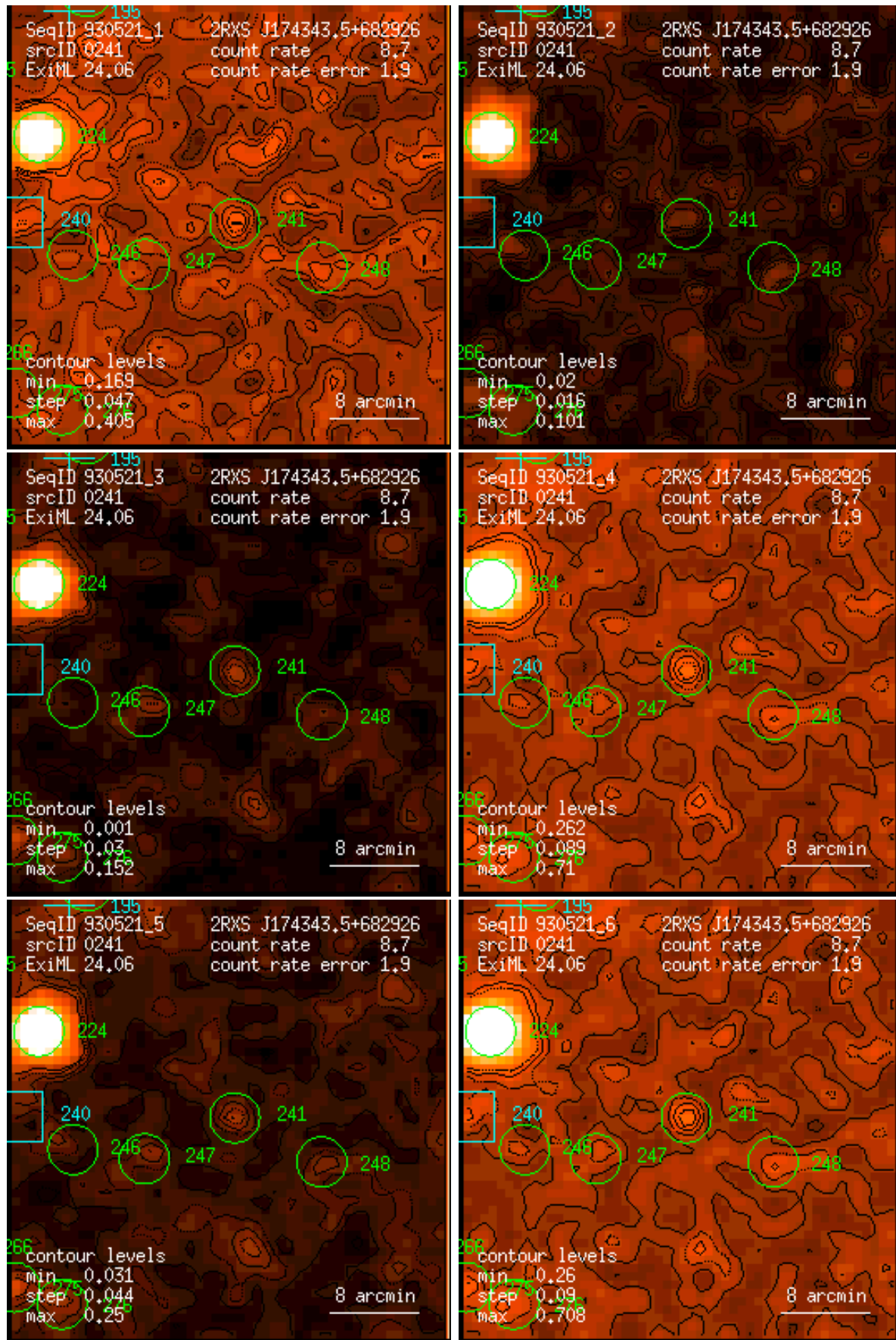
Figure 241: RASS 930521: detection 0241: band rate images, Gaussian filter: (1) PSPC channels 11 – 41, (2) 52 – 90, (3) 91 – 201, (4) 11 – 235, (5) 52 – 201, (6) 11 – 201. Broad band rates in counts/ks. Band rate contour levels in counts/ks/arcmin 2 .
