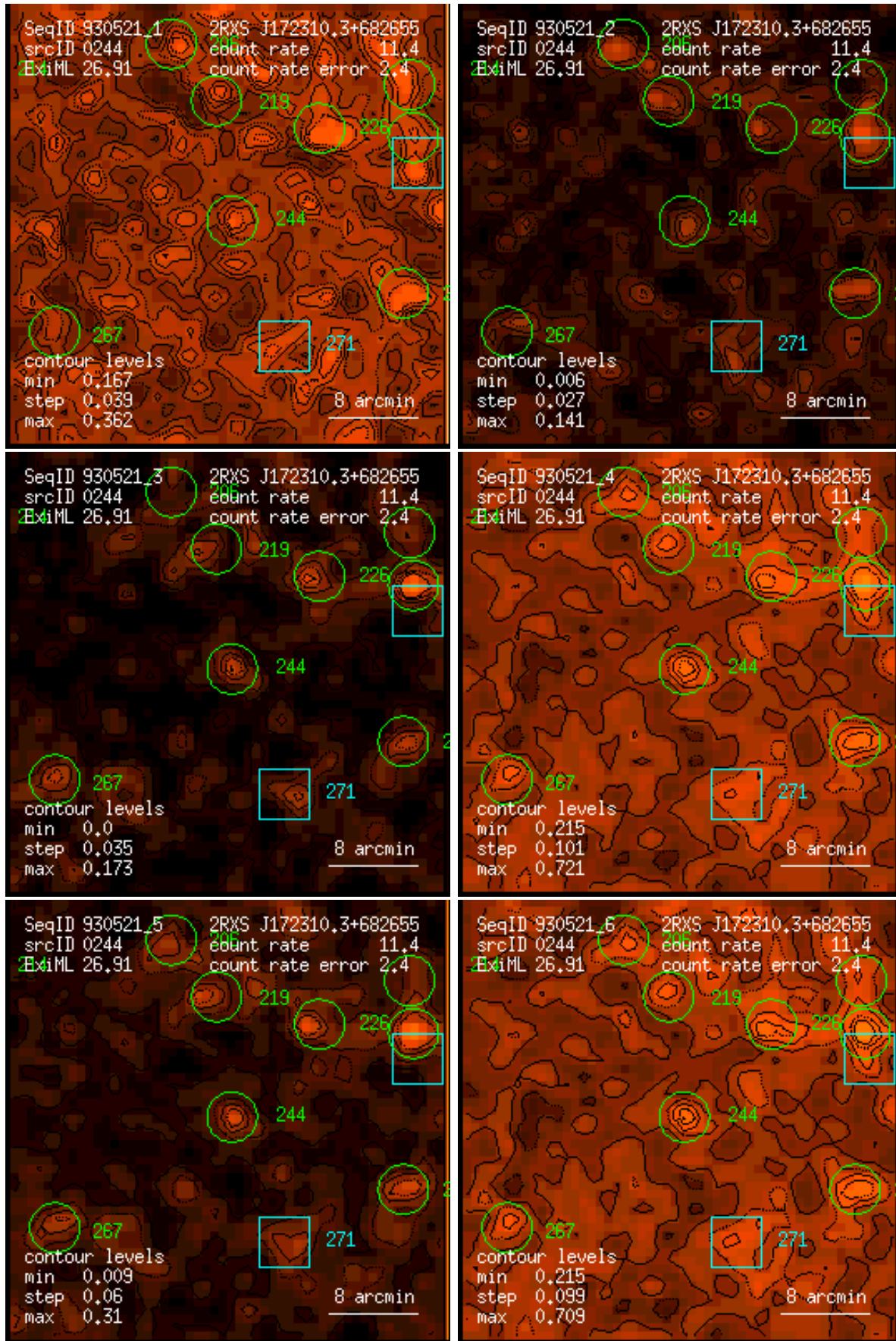
Figure 244: RASS 930521: detection 0244: band rate images, Gaussian filter: (1) PSPC channels 11 – 41, (2) 52 – 90, (3) 91 – 201, (4) 11 – 235, (5) 52 – 201, (6) 11 – 201. Broad band rates in counts/ks. Band rate contour levels in counts/ks/arcmin 2 .
