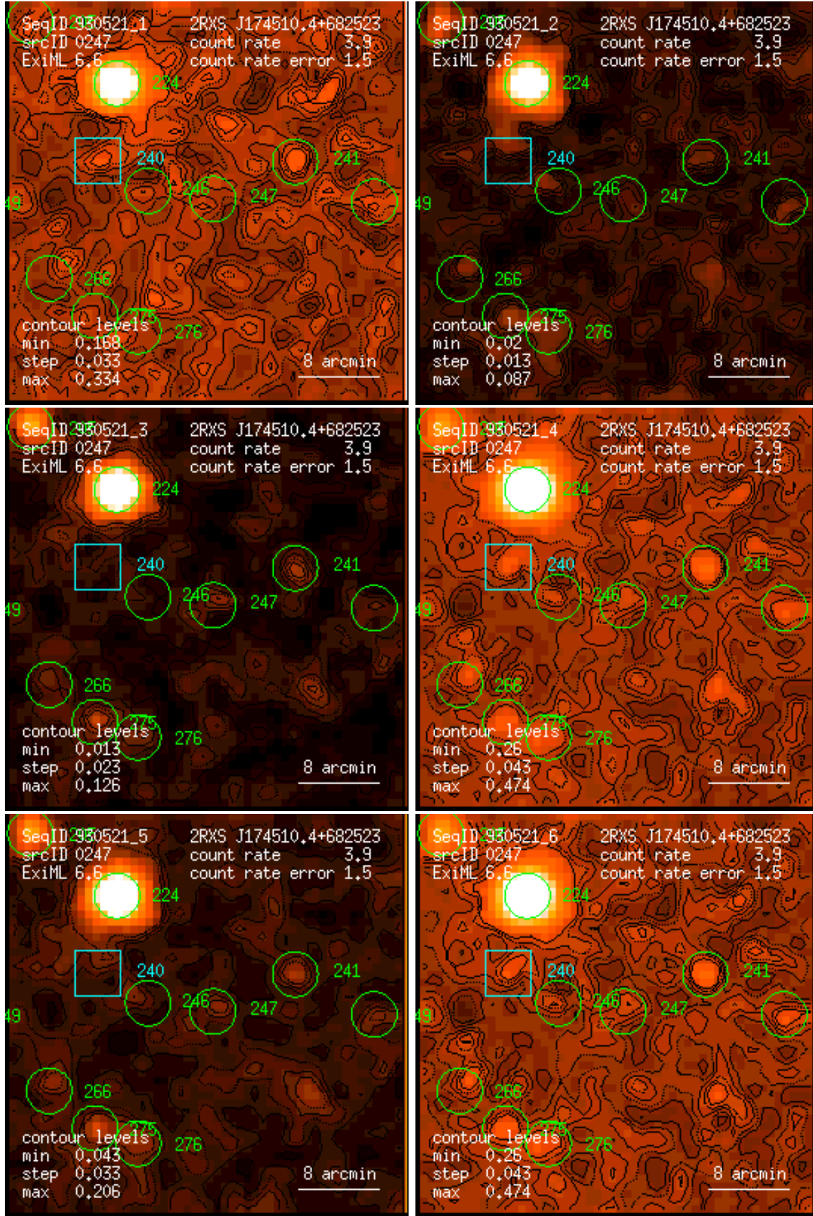
Figure 247: RASS 930521: detection 0247: band rate images, Gaussian filter: (1) PSPC channels 11 – 41, (2) 52 – 90, (3) 91 – 201, (4) 11 – 235, (5) 52 – 201, (6) 11 – 201. Broad band rates in counts/ks. Band rate contour levels in counts/ks/arcmin 2 .
