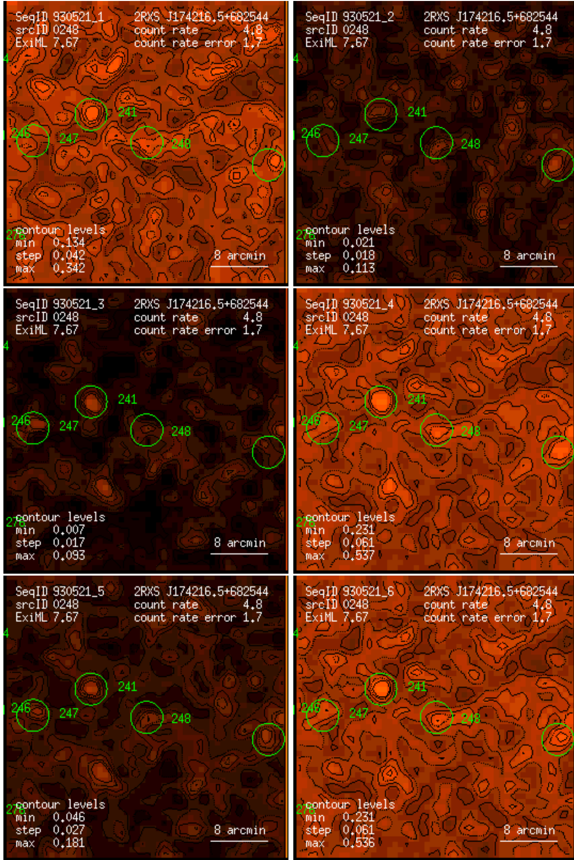
Figure 248: RASS 930521: detection 0248: band rate images, Gaussian filter: (1) PSPC channels 11 – 41, (2) 52 – 90, (3) 91 – 201, (4) 11 – 235, (5) 52 – 201, (6) 11 – 201. Broad band rates in counts/ks. Band rate contour levels in counts/ks/arcmin 2 .
