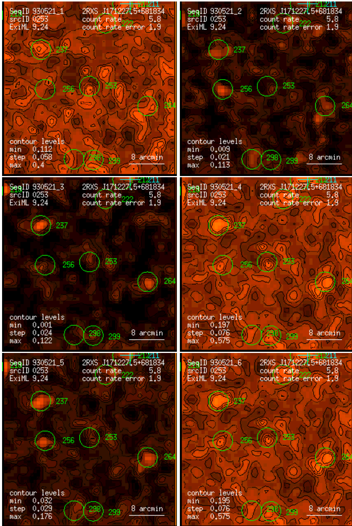
Figure 253: RASS 930521: detection 0253: band rate images, Gaussian filter: (1) PSPC channels 11 – 41, (2) 52 – 90, (3) 91 – 201, (4) 11 – 235, (5) 52 – 201, (6) 11 – 201. Broad band rates in counts/ks. Band rate contour levels in counts/ks/arcmin 2 .
