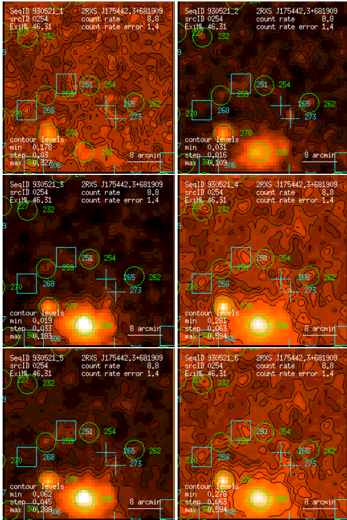
Figure 254: RASS 930521: detection 0254: band rate images, Gaussian filter: (1) PSPC channels 11 – 41, (2) 52 – 90, (3) 91 – 201, (4) 11 – 235, (5) 52 – 201, (6) 11 – 201. Broad band rates in counts/ks. Band rate contour levels in counts/ks/arcmin 2 .
