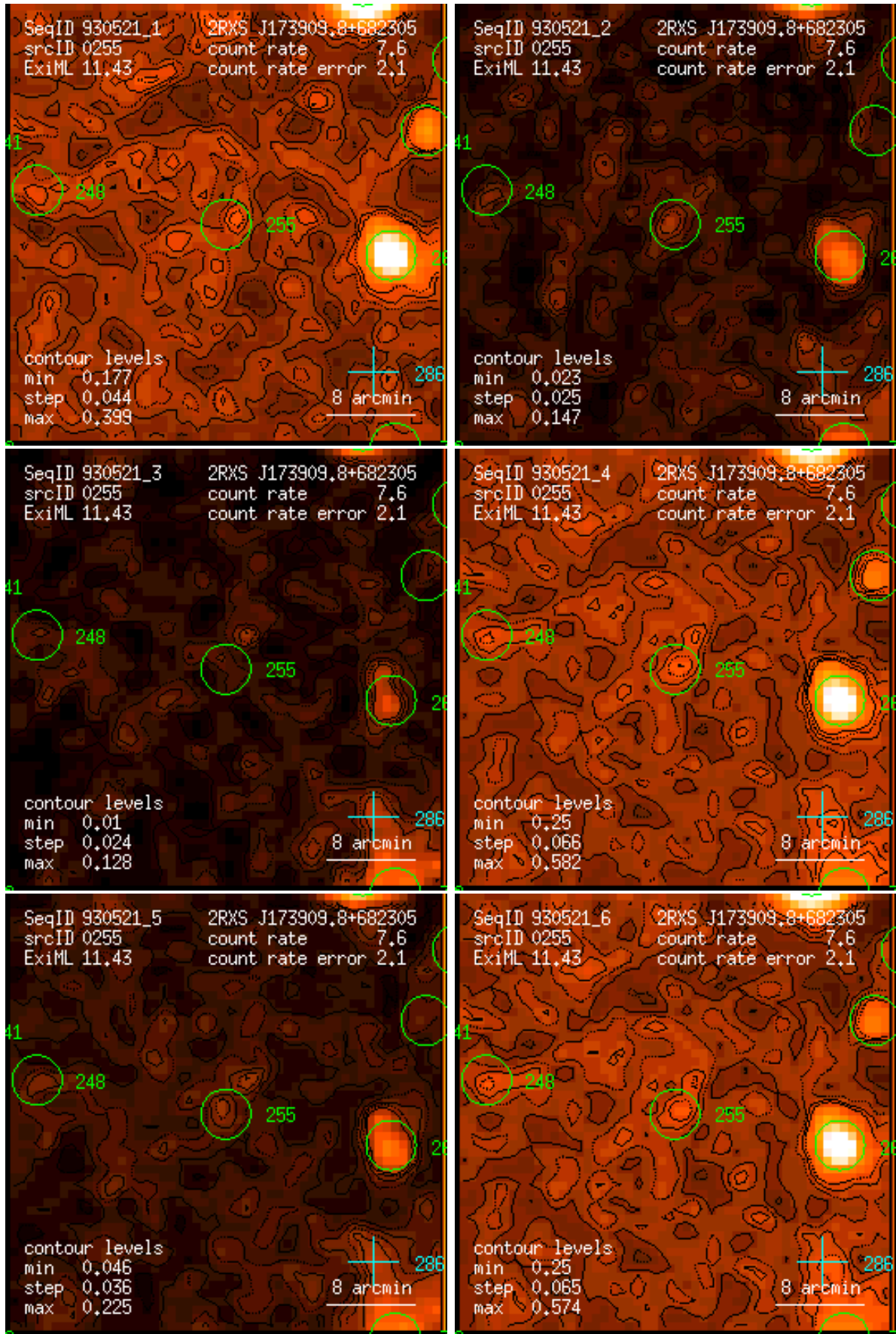
Figure 255: RASS 930521: detection 0255: band rate images, Gaussian filter: (1) PSPC channels 11 – 41, (2) 52 – 90, (3) 91 – 201, (4) 11 – 235, (5) 52 – 201, (6) 11 – 201. Broad band rates in counts/ks. Band rate contour levels in counts/ks/arcmin 2 .
