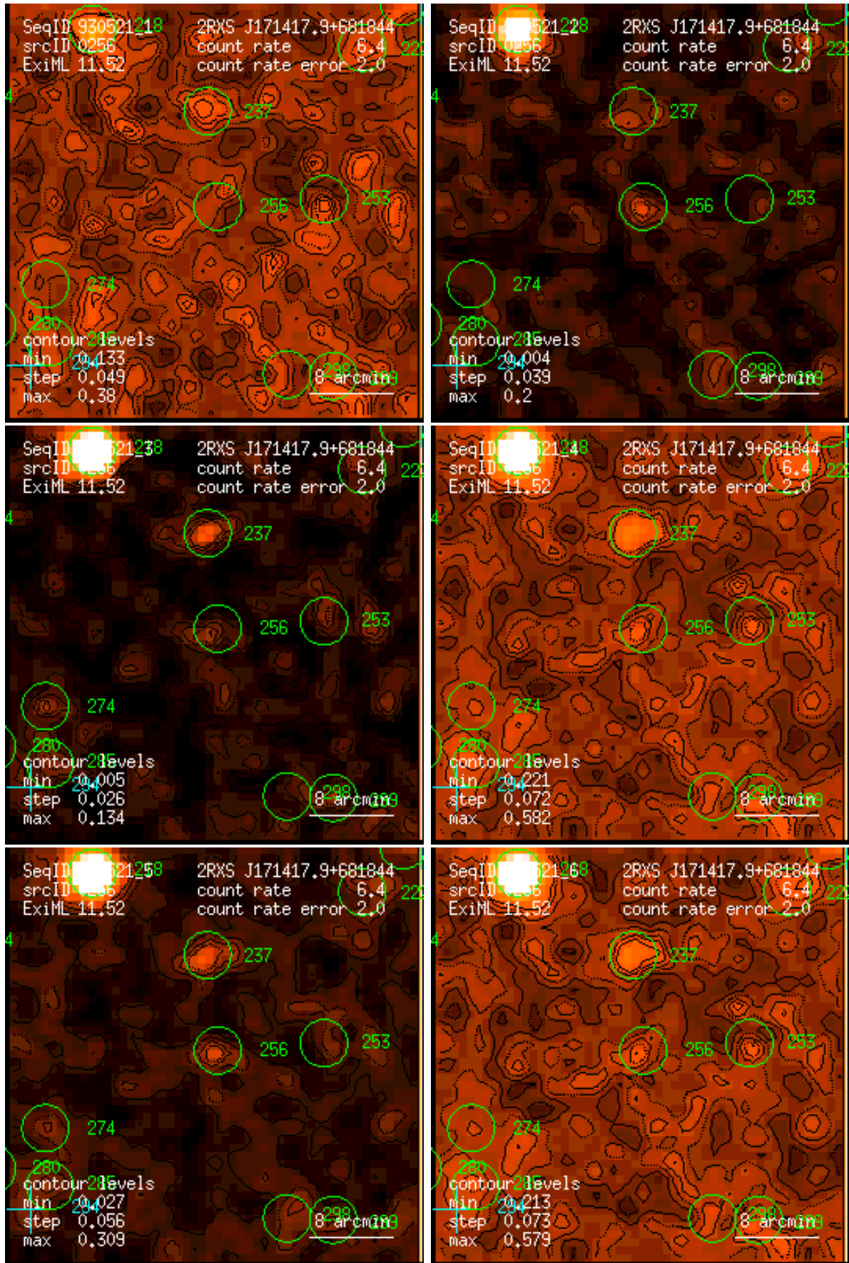
Figure 256: RASS 930521: detection 0256: band rate images, Gaussian filter: (1) PSPC channels 11 – 41, (2) 52 – 90, (3) 91 – 201, (4) 11 – 235, (5) 52 – 201, (6) 11 – 201. Broad band rates in counts/ks. Band rate contour levels in counts/ks/arcmin 2 .
