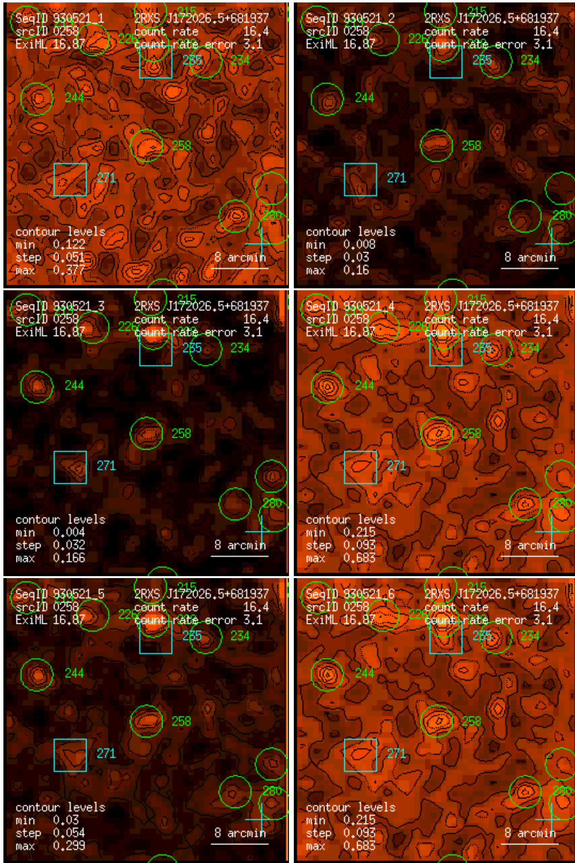
Figure 258: RASS 930521: detection 0258: band rate images, Gaussian filter: (1) PSPC channels 11 – 41, (2) 52 – 90, (3) 91 – 201, (4) 11 – 235, (5) 52 – 201, (6) 11 – 201. Broad band rates in counts/ks. Band rate contour levels in counts/ks/arcmin 2 .
