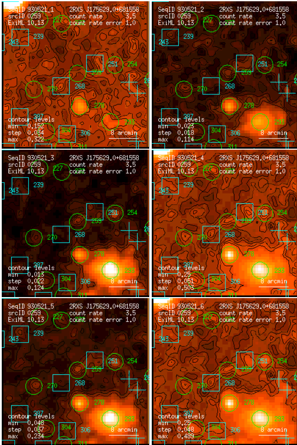
Figure 259: RASS 930521: detection 0259: band rate images, Gaussian filter: (1) PSPC channels 11 – 41, (2) 52 – 90, (3) 91 – 201, (4) 11 – 235, (5) 52 – 201, (6) 11 – 201. Broad band rates in counts/ks. Band rate contour levels in counts/ks/arcmin 2 .
