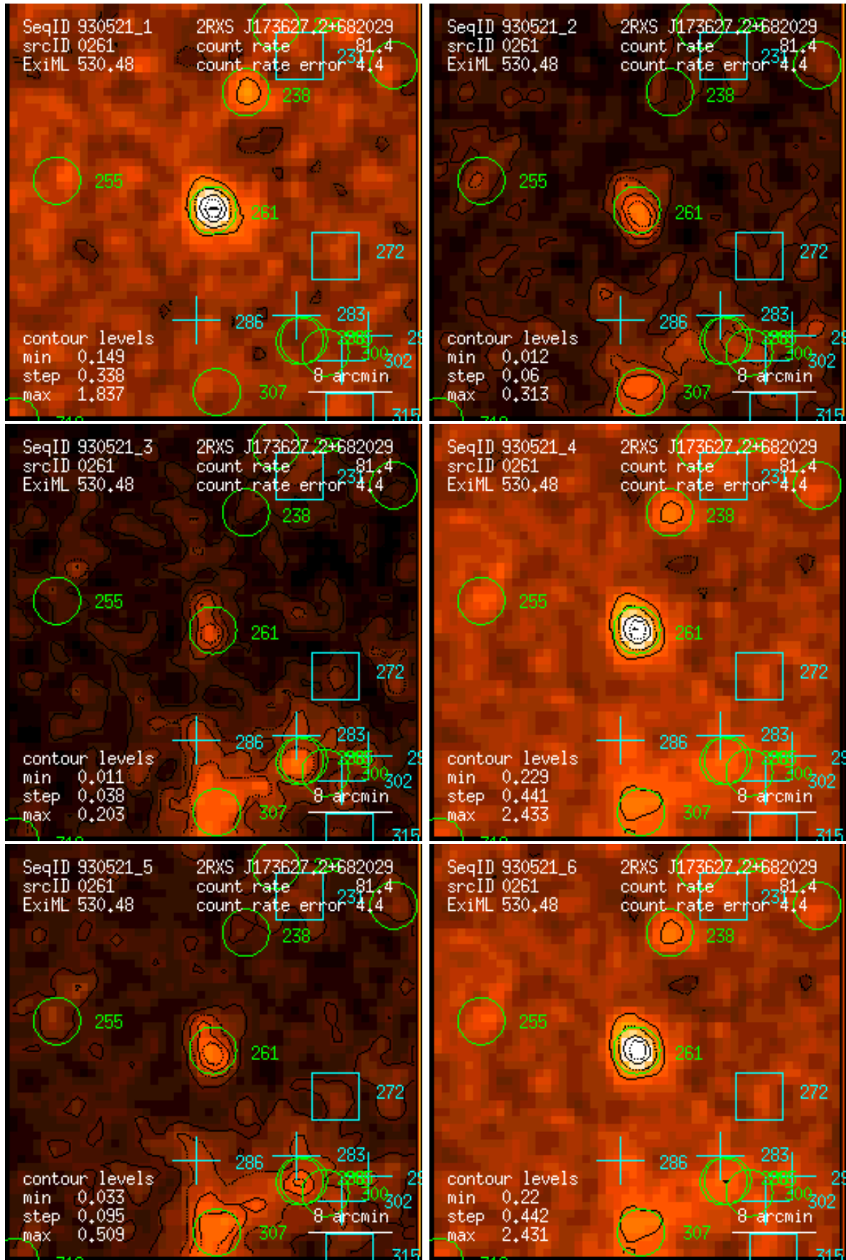
Figure 261: RASS 930521: detection 0261: band rate images, Gaussian filter: (1) PSPC channels 11 – 41, (2) 52 – 90, (3) 91 – 201, (4) 11 – 235, (5) 52 – 201, (6) 11 – 201. Broad band rates in counts/ks. Band rate contour levels in counts/ks/arcmin 2 .
