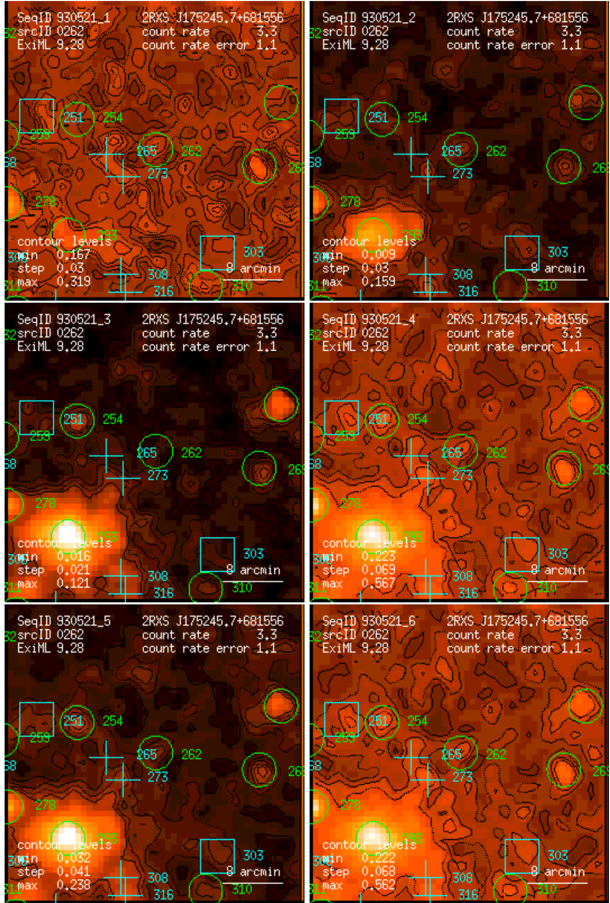
Figure 262: RASS 930521: detection 0262: band rate images, Gaussian filter: (1) PSPC channels 11 – 41, (2) 52 – 90, (3) 91 – 201, (4) 11 – 235, (5) 52 – 201, (6) 11 – 201. Broad band rates in counts/ks. Band rate contour levels in counts/ks/arcmin 2 .
