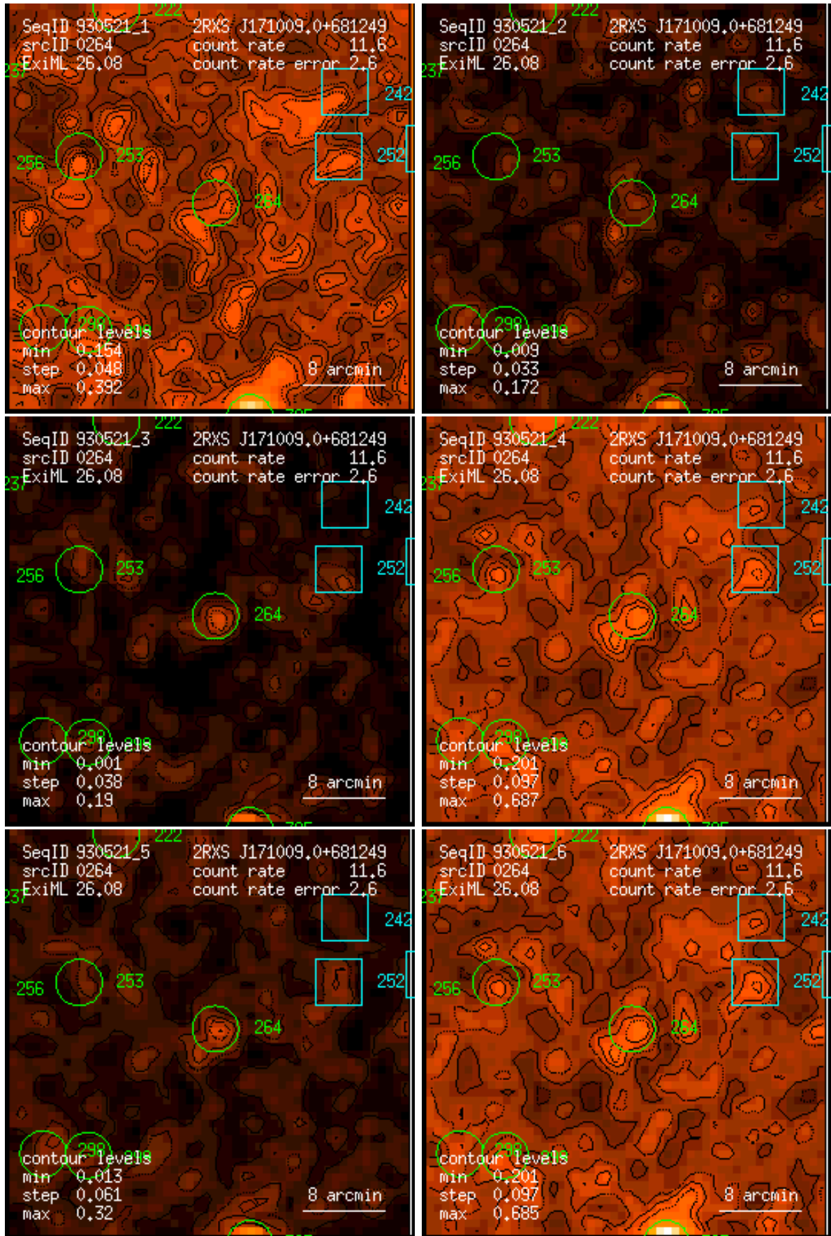
Figure 264: RASS 930521: detection 0264: band rate images, Gaussian filter: (1) PSPC channels 11 – 41, (2) 52 – 90, (3) 91 – 201, (4) 11 – 235, (5) 52 – 201, (6) 11 – 201. Broad band rates in counts/ks. Band rate contour levels in counts/ks/arcmin 2 .
