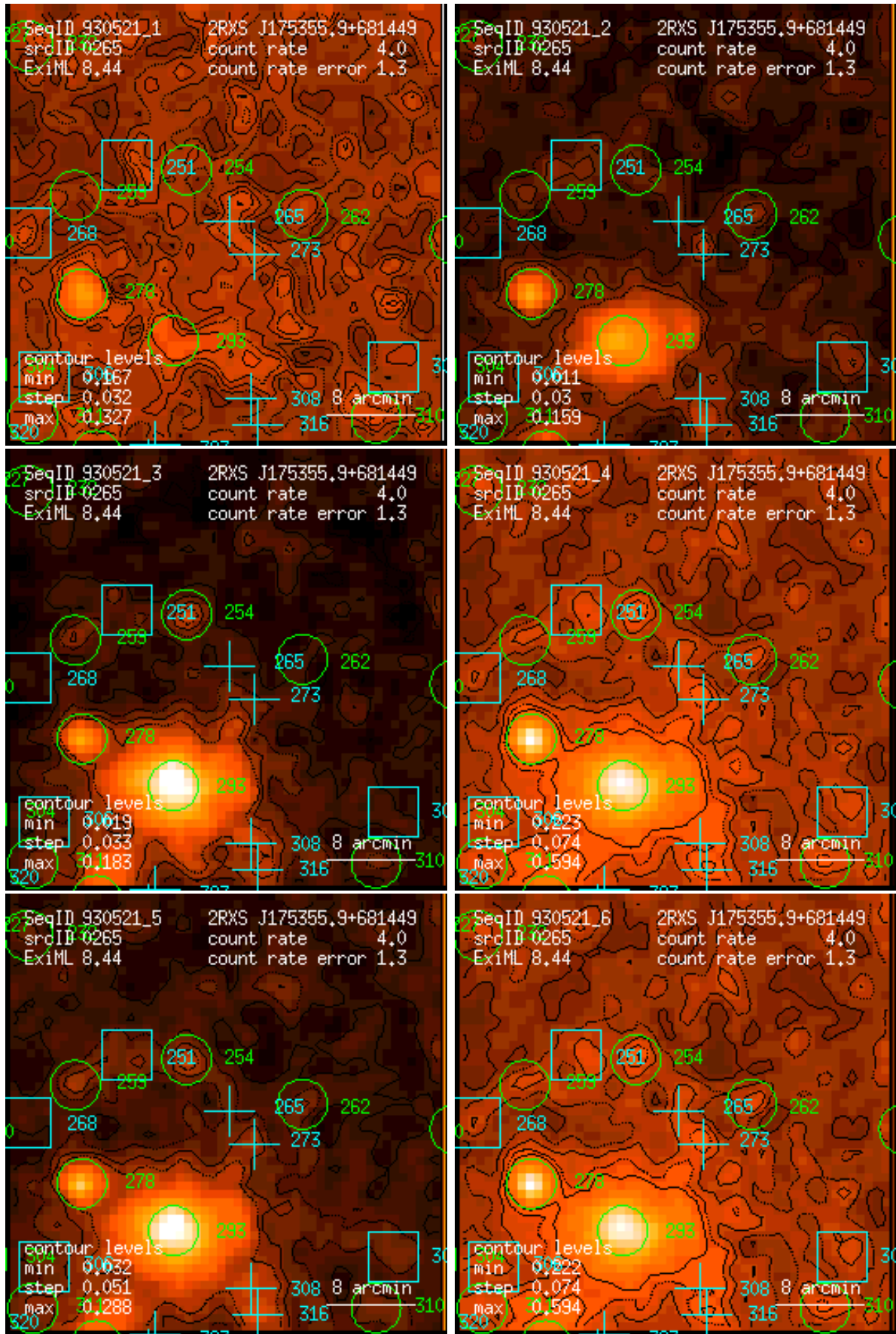
Figure 265: RASS 930521: detection 0265: band rate images, Gaussian filter: (1) PSPC channels 11 – 41, (2) 52 – 90, (3) 91 – 201, (4) 11 – 235, (5) 52 – 201, (6) 11 – 201. Broad band rates in counts/ks. Band rate contour levels in counts/ks/arcmin 2 .
