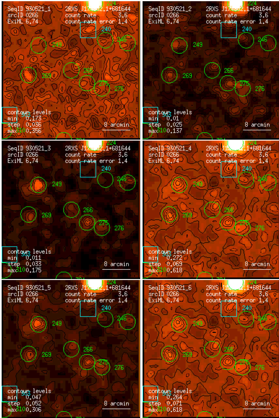
Figure 266: RASS 930521: detection 0266: band rate images, Gaussian filter: (1) PSPC channels 11 – 41, (2) 52 – 90, (3) 91 – 201, (4) 11 – 235, (5) 52 – 201, (6) 11 – 201. Broad band rates in counts/ks. Band rate contour levels in counts/ks/arcmin 2 .
