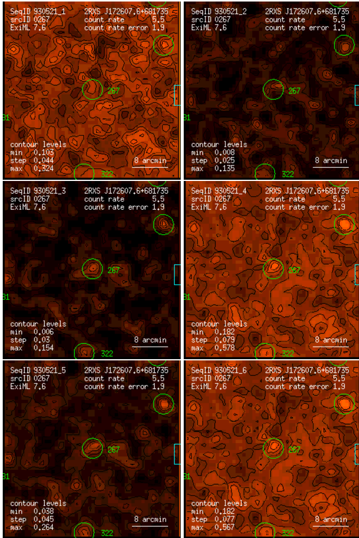
Figure 267: RASS 930521: detection 0267: band rate images, Gaussian filter: (1) PSPC channels 11 – 41, (2) 52 – 90, (3) 91 – 201, (4) 11 – 235, (5) 52 – 201, (6) 11 – 201. Broad band rates in counts/ks. Band rate contour levels in counts/ks/arcmin 2 .
