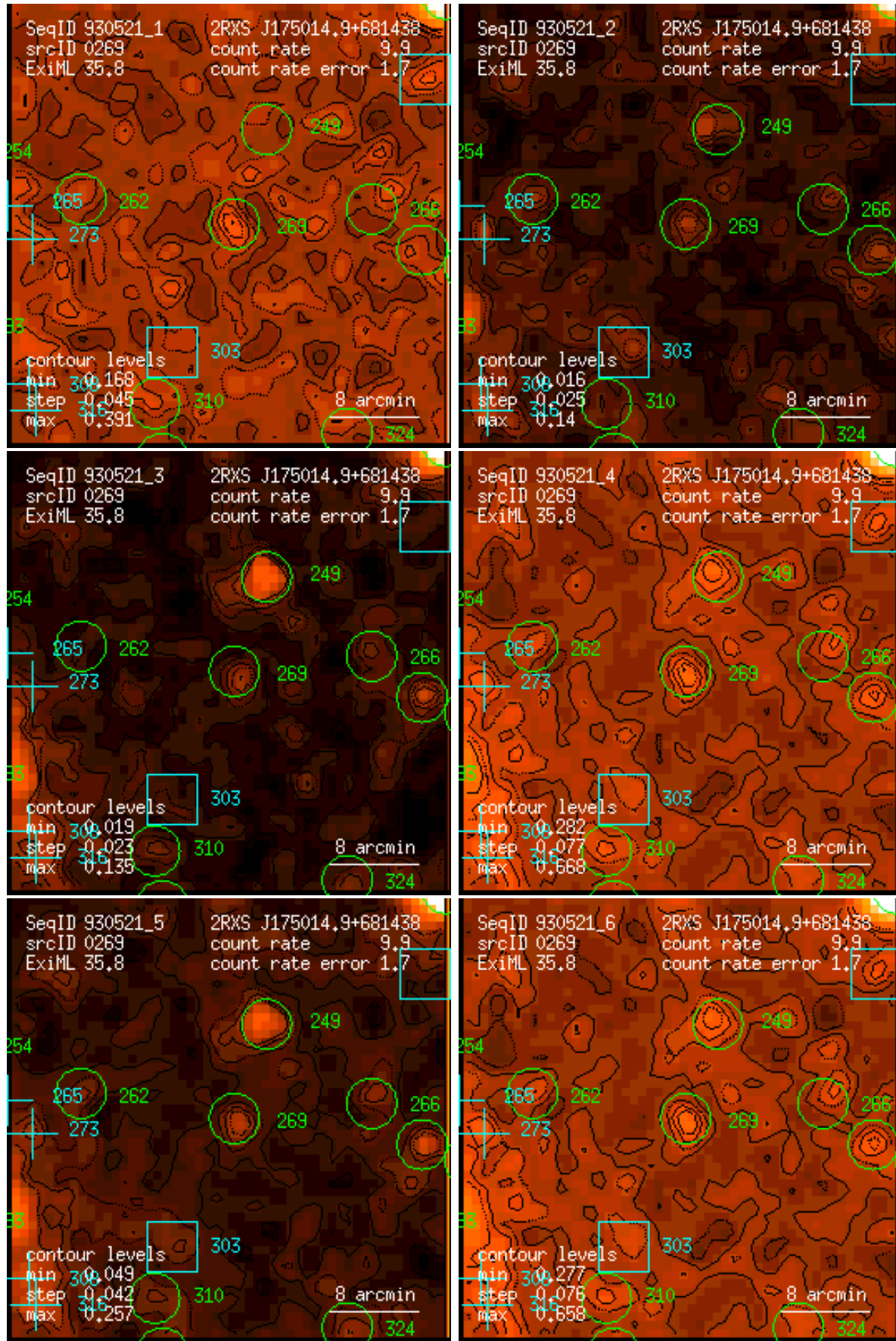
Figure 269: RASS 930521: detection 0269: band rate images, Gaussian filter: (1) PSPC channels 11 – 41, (2) 52 – 90, (3) 91 – 201, (4) 11 – 235, (5) 52 – 201, (6) 11 – 201. Broad band rates in counts/ks. Band rate contour levels in counts/ks/arcmin 2 .
