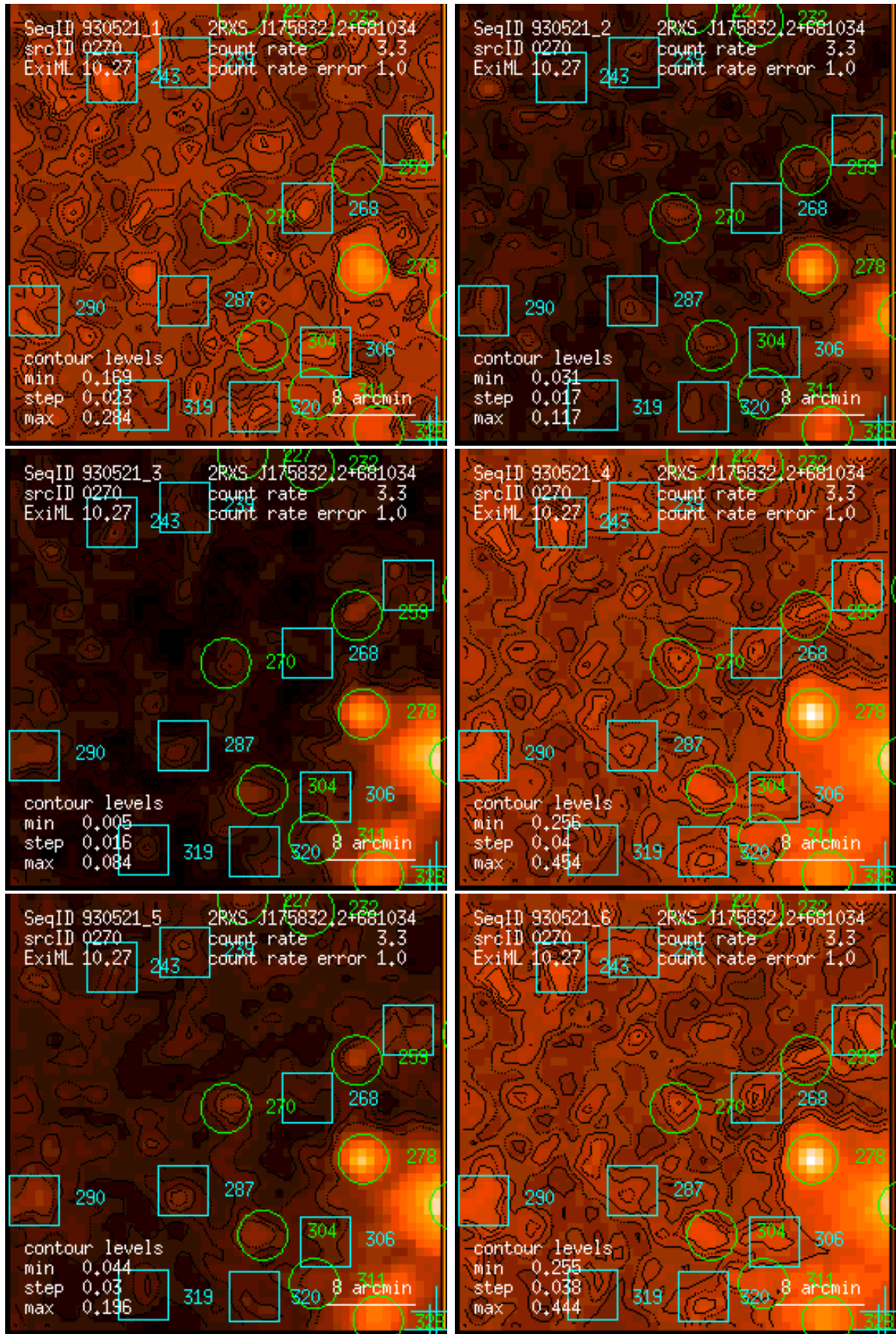
Figure 270: RASS 930521: detection 0270: band rate images, Gaussian filter: (1) PSPC channels 11 – 41, (2) 52 – 90, (3) 91 – 201, (4) 11 – 235, (5) 52 – 201, (6) 11 – 201. Broad band rates in counts/ks. Band rate contour levels in counts/ks/arcmin 2 .
