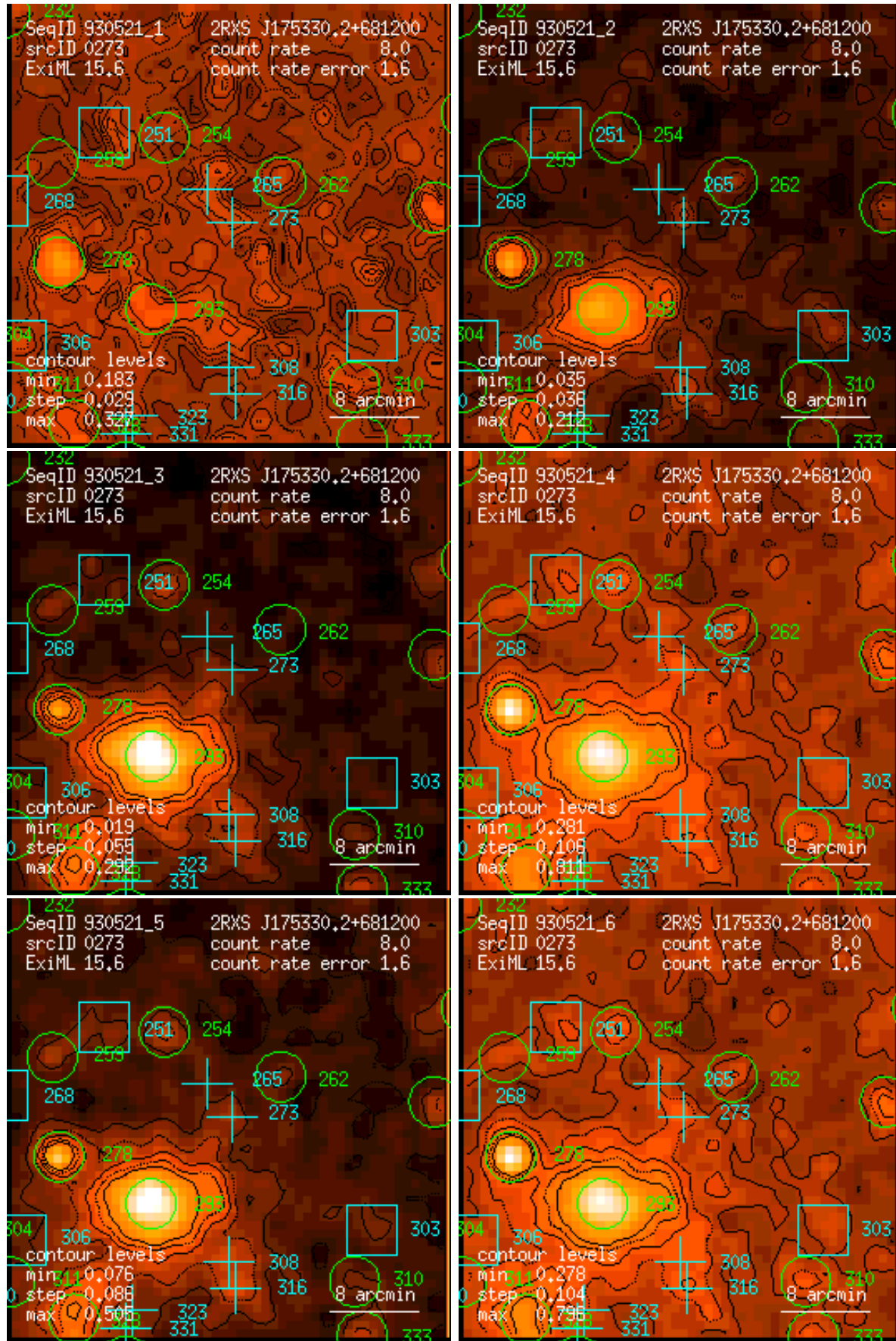
Figure 273: RASS 930521: detection 0273: band rate images, Gaussian filter: (1) PSPC channels 11 – 41, (2) 52 – 90, (3) 91 – 201, (4) 11 – 235, (5) 52 – 201, (6) 11 – 201. Broad band rates in counts/ks. Band rate contour levels in counts/ks/arcmin 2 .
