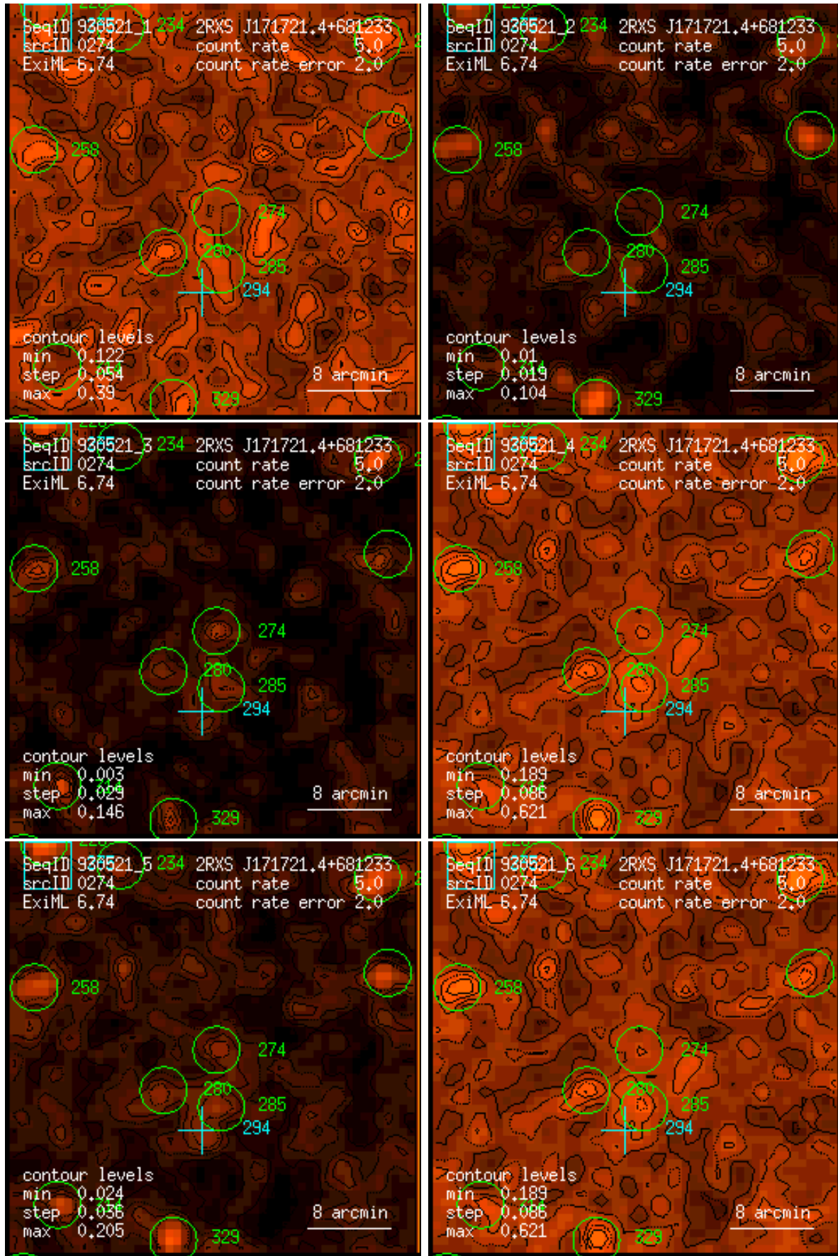
Figure 274: RASS 930521: detection 0274: band rate images, Gaussian filter: (1) PSPC channels 11 – 41, (2) 52 – 90, (3) 91 – 201, (4) 11 – 235, (5) 52 – 201, (6) 11 – 201. Broad band rates in counts/ks. Band rate contour levels in counts/ks/arcmin 2 .
