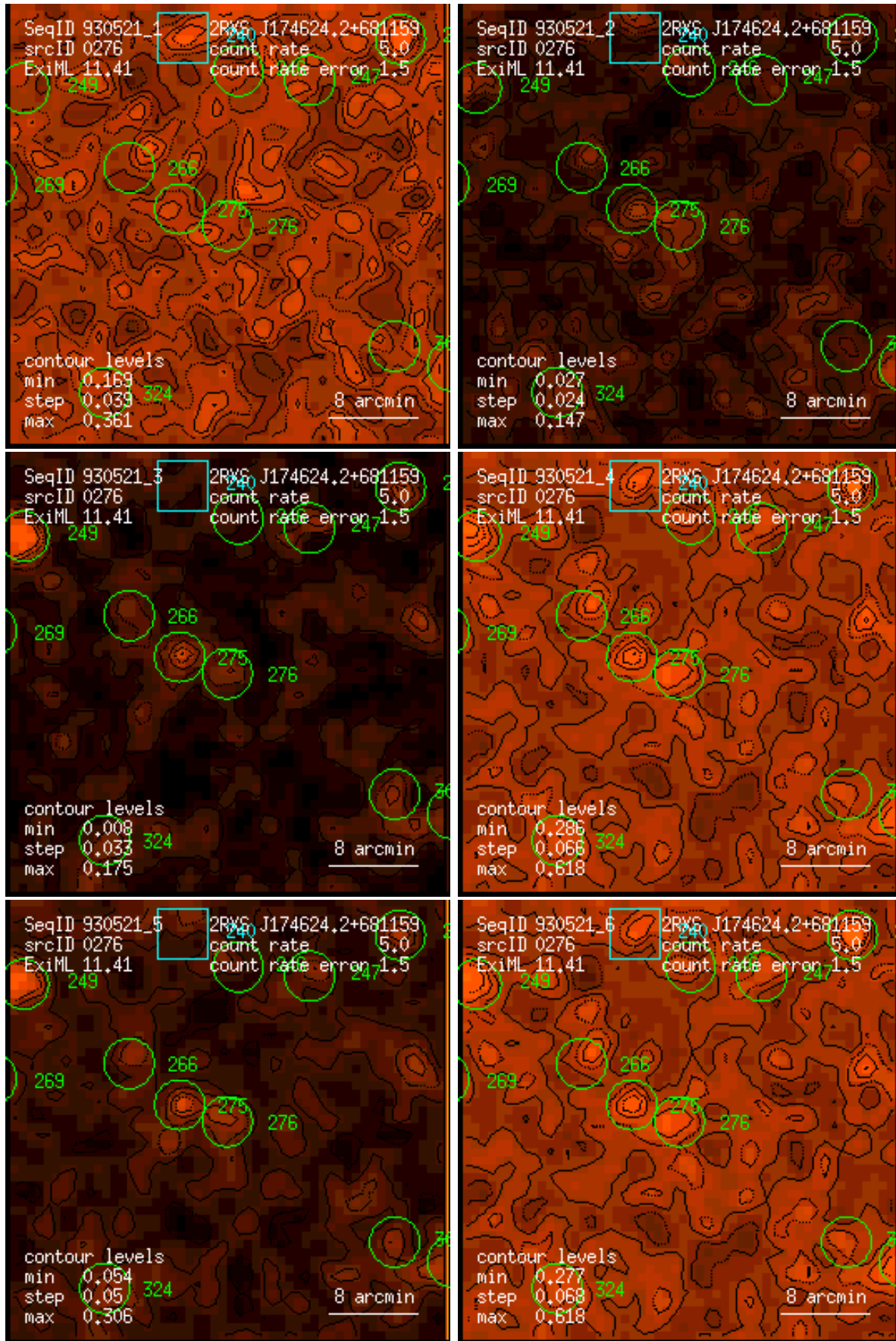
Figure 276: RASS 930521: detection 0276: band rate images, Gaussian filter: (1) PSPC channels 11 – 41, (2) 52 – 90, (3) 91 – 201, (4) 11 – 235, (5) 52 – 201, (6) 11 – 201. Broad band rates in counts/ks. Band rate contour levels in counts/ks/arcmin 2 .
