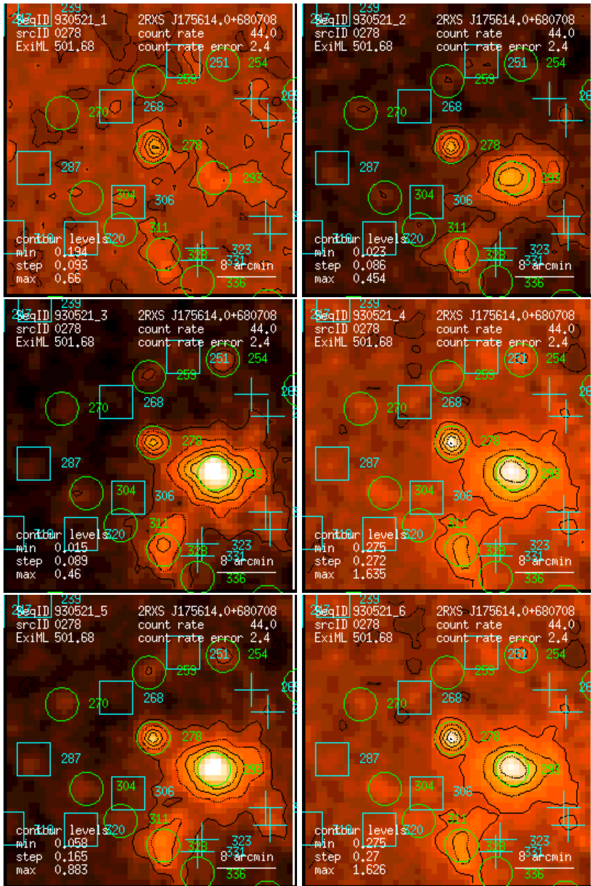
Figure 278: RASS 930521: detection 0278: band rate images, Gaussian filter: (1) PSPC channels 11 – 41, (2) 52 – 90, (3) 91 – 201, (4) 11 – 235, (5) 52 – 201, (6) 11 – 201. Broad band rates in counts/ks. Band rate contour levels in counts/ks/arcmin 2 .
