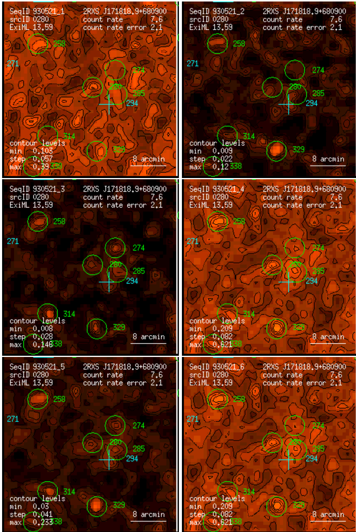
Figure 280: RASS 930521: detection 0280: band rate images, Gaussian filter: (1) PSPC channels 11 – 41, (2) 52 – 90, (3) 91 – 201, (4) 11 – 235, (5) 52 – 201, (6) 11 – 201. Broad band rates in counts/ks. Band rate contour levels in counts/ks/arcmin 2 .
