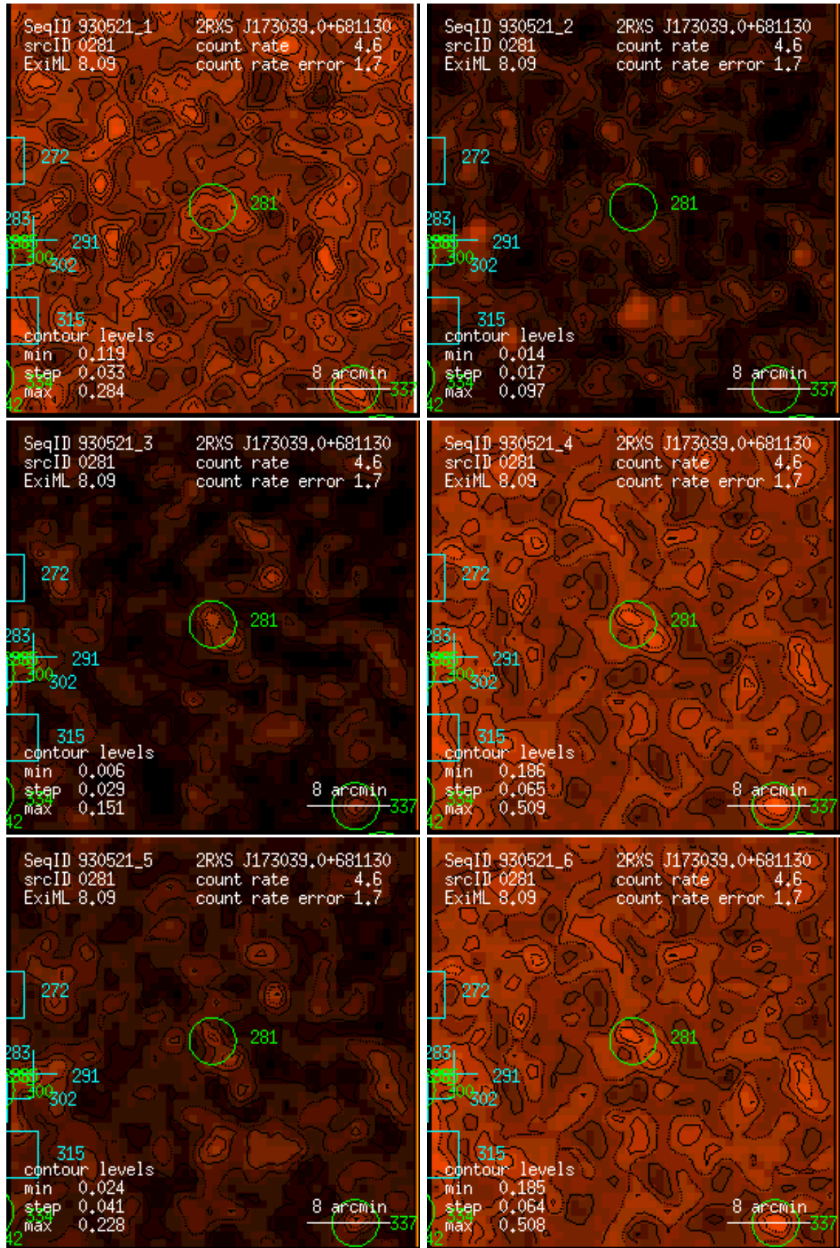
Figure 281: RASS 930521: detection 0281: band rate images, Gaussian filter: (1) PSPC channels 11 – 41, (2) 52 – 90, (3) 91 – 201, (4) 11 – 235, (5) 52 – 201, (6) 11 – 201. Broad band rates in counts/ks. Band rate contour levels in counts/ks/arcmin 2 .
