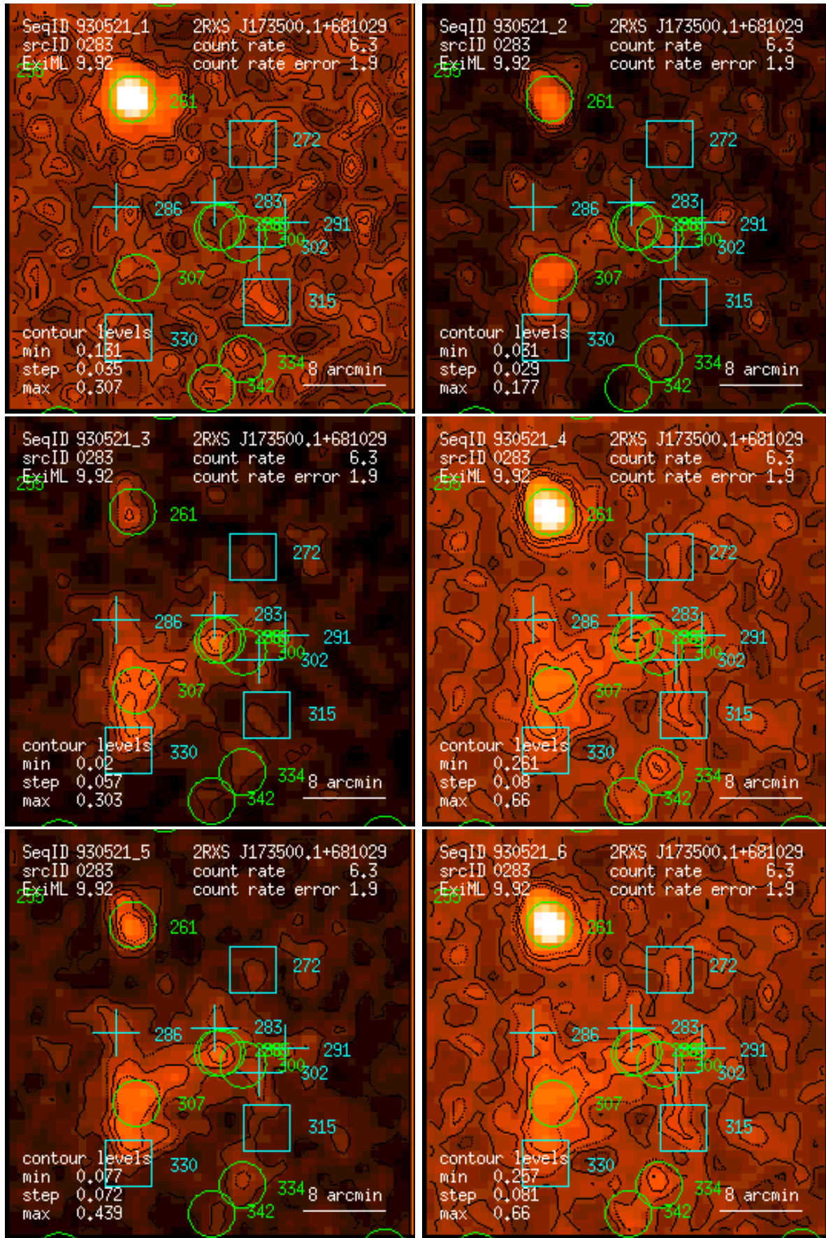
Figure 283: RASS 930521: detection 0283: band rate images, Gaussian filter: (1) PSPC channels 11 – 41, (2) 52 – 90, (3) 91 – 201, (4) 11 – 235, (5) 52 – 201, (6) 11 – 201. Broad band rates in counts/ks. Band rate contour levels in counts/ks/arcmin 2 .
