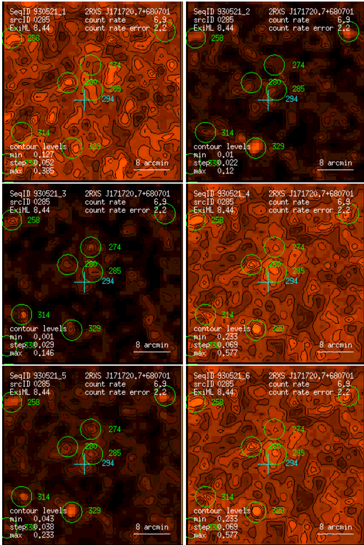
Figure 285: RASS 930521: detection 0285: band rate images, Gaussian filter: (1) PSPC channels 11 – 41, (2) 52 – 90, (3) 91 – 201, (4) 11 – 235, (5) 52 – 201, (6) 11 – 201. Broad band rates in counts/ks. Band rate contour levels in counts/ks/arcmin 2 .
