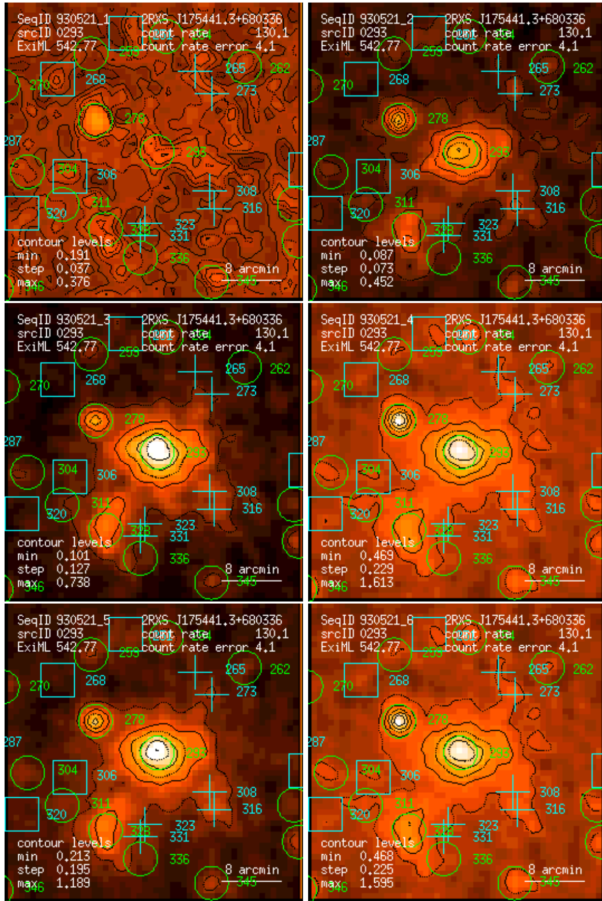
Figure 293: RASS 930521: detection 0293: band rate images, Gaussian filter: (1) PSPC channels 11 – 41, (2) 52 – 90, (3) 91 – 201, (4) 11 – 235, (5) 52 – 201, (6) 11 – 201. Broad band rates in counts/ks. Band rate contour levels in counts/ks/arcmin 2 .
