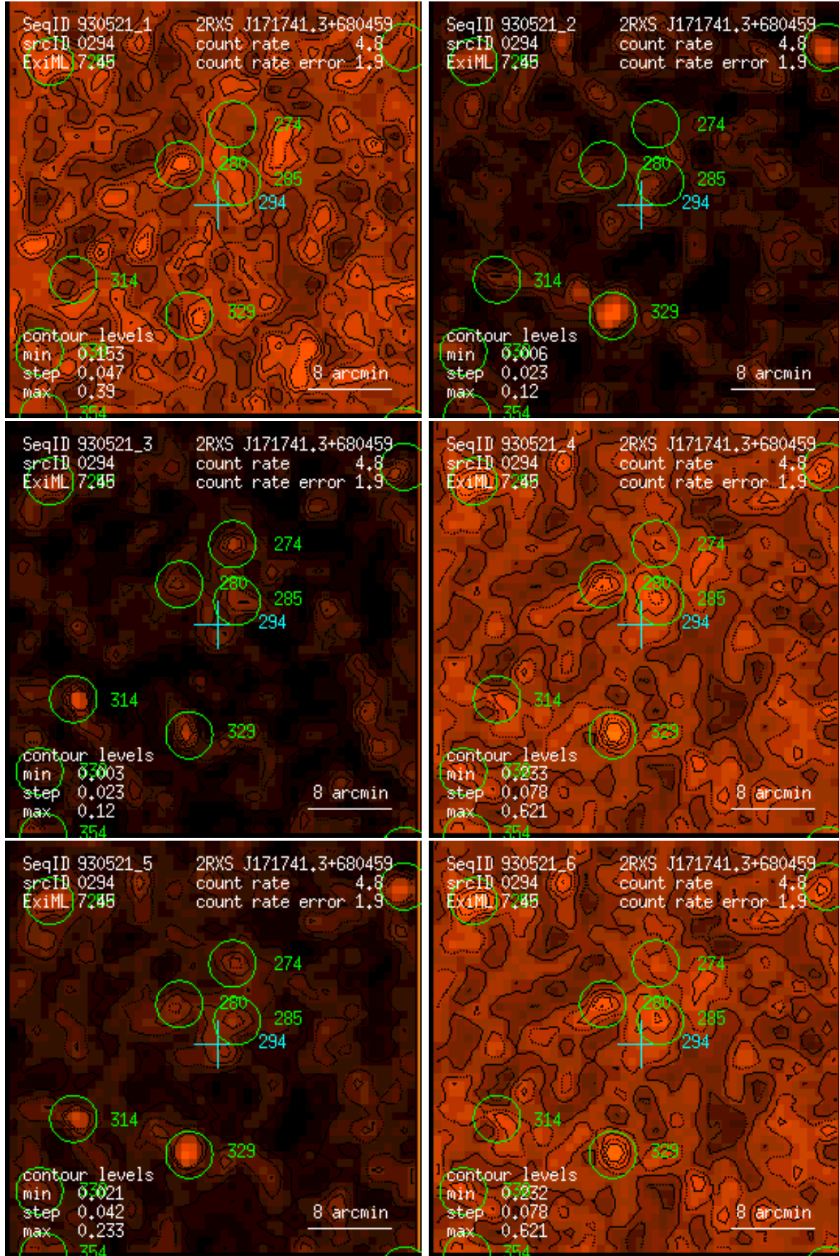
Figure 294: RASS 930521: detection 0294: band rate images, Gaussian filter: (1) PSPC channels 11 – 41, (2) 52 – 90, (3) 91 – 201, (4) 11 – 235, (5) 52 – 201, (6) 11 – 201. Broad band rates in counts/ks. Band rate contour levels in counts/ks/arcmin 2 .
