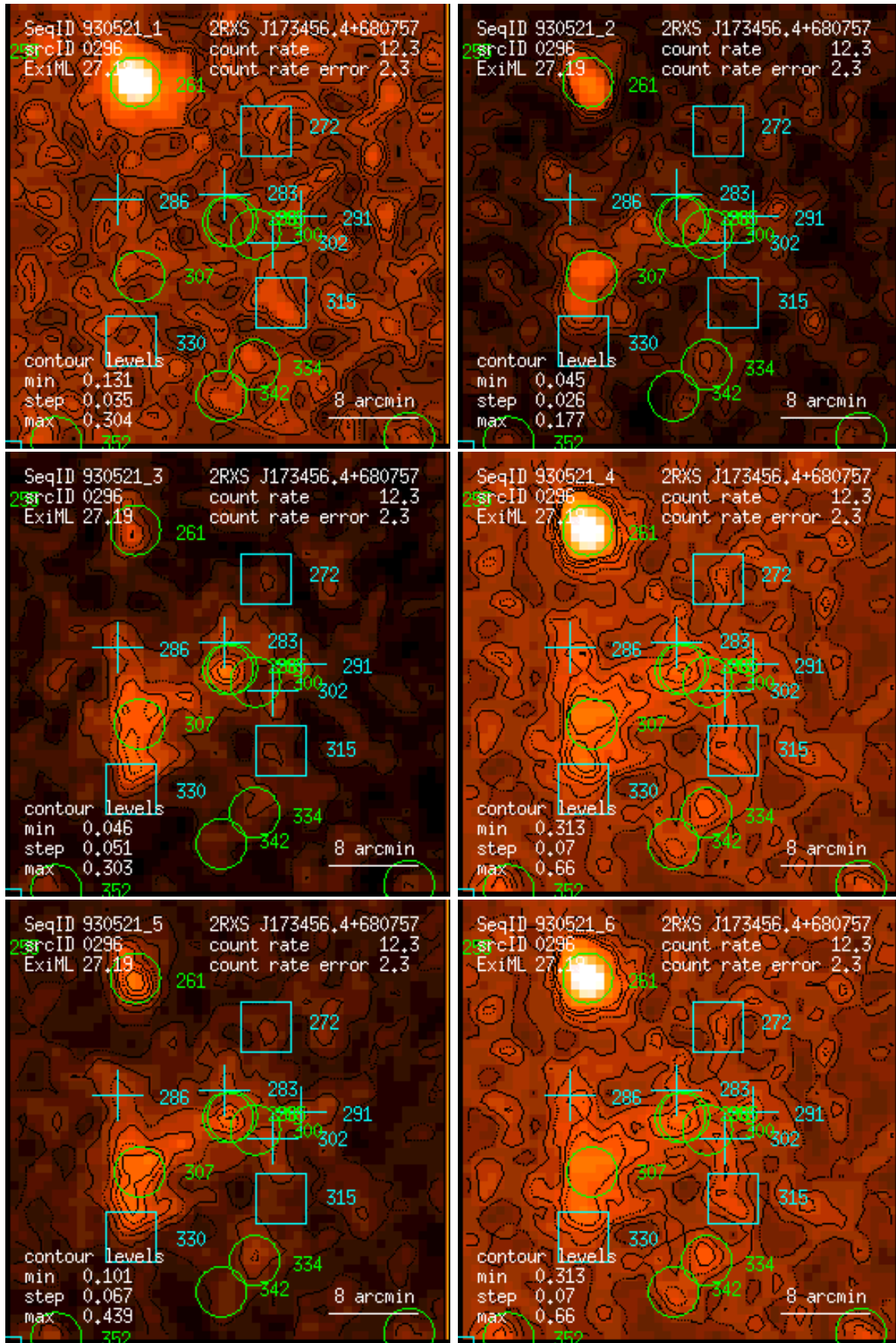
Figure 296: RASS 930521: detection 0296: band rate images, Gaussian filter: (1) PSPC channels 11 – 41, (2) 52 – 90, (3) 91 – 201, (4) 11 – 235, (5) 52 – 201, (6) 11 – 201. Broad band rates in counts/ks. Band rate contour levels in counts/ks/arcmin 2 .
