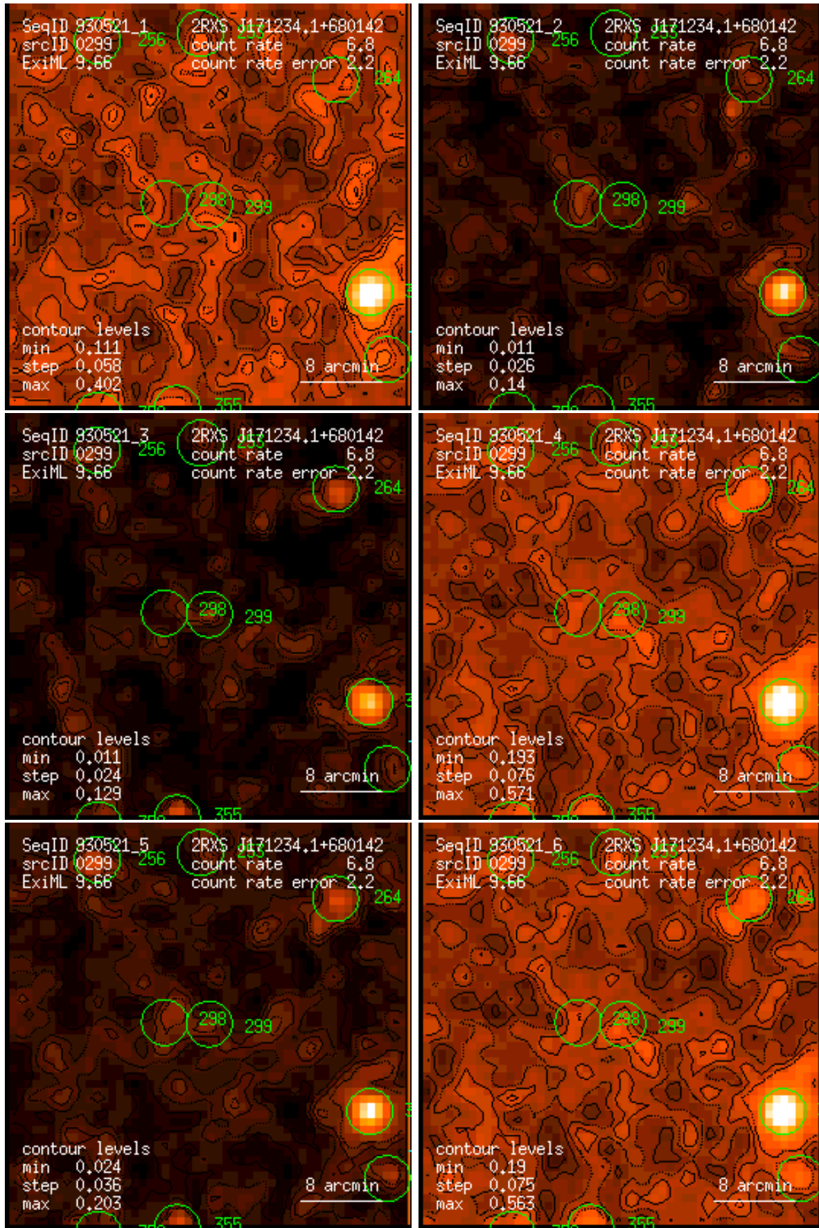
Figure 299: RASS 930521: detection 0299: band rate images, Gaussian filter: (1) PSPC channels 11 – 41, (2) 52 – 90, (3) 91 – 201, (4) 11 – 235, (5) 52 – 201, (6) 11 – 201. Broad band rates in counts/ks. Band rate contour levels in counts/ks/arcmin 2 .
