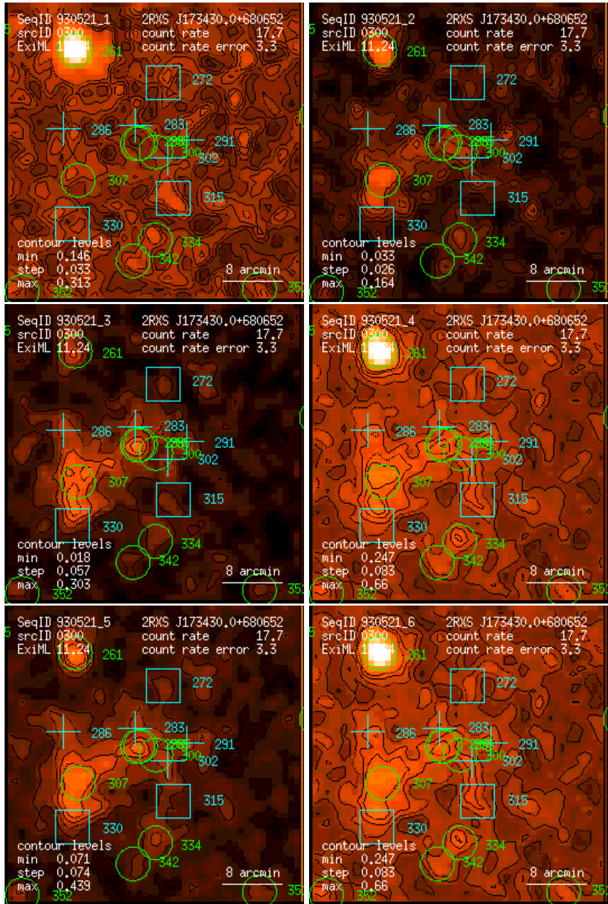
Figure 300: RASS 930521: detection 0300: band rate images, Gaussian filter: (1) PSPC channels 11 – 41, (2) 52 – 90, (3) 91 – 201, (4) 11 – 235, (5) 52 – 201, (6) 11 – 201. Broad band rates in counts/ks. Band rate contour levels in counts/ks/arcmin 2 .
