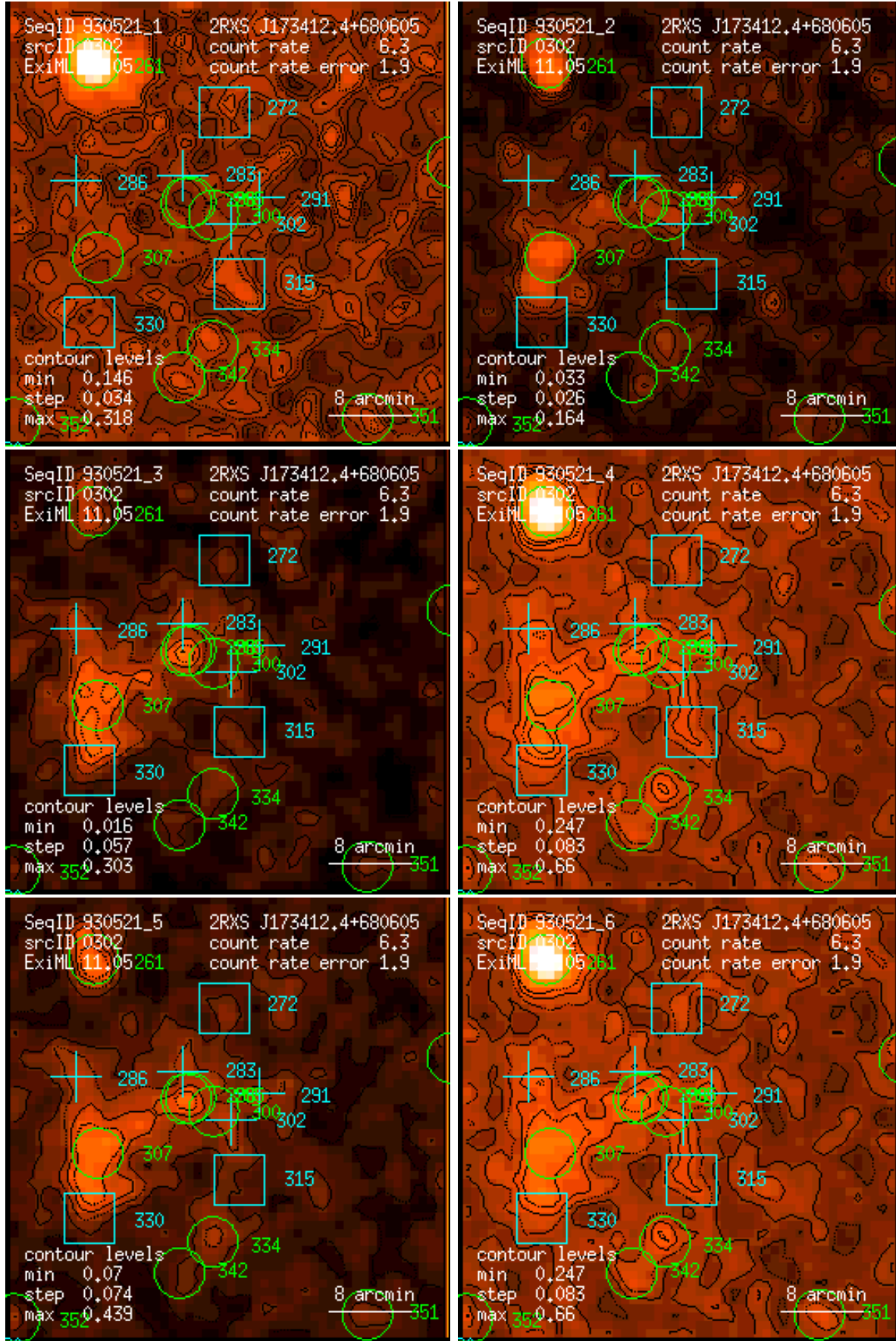
Figure 302: RASS 930521: detection 0302: band rate images, Gaussian filter: (1) PSPC channels 11 – 41, (2) 52 – 90, (3) 91 – 201, (4) 11 – 235, (5) 52 – 201, (6) 11 – 201. Broad band rates in counts/ks. Band rate contour levels in counts/ks/arcmin 2 .
