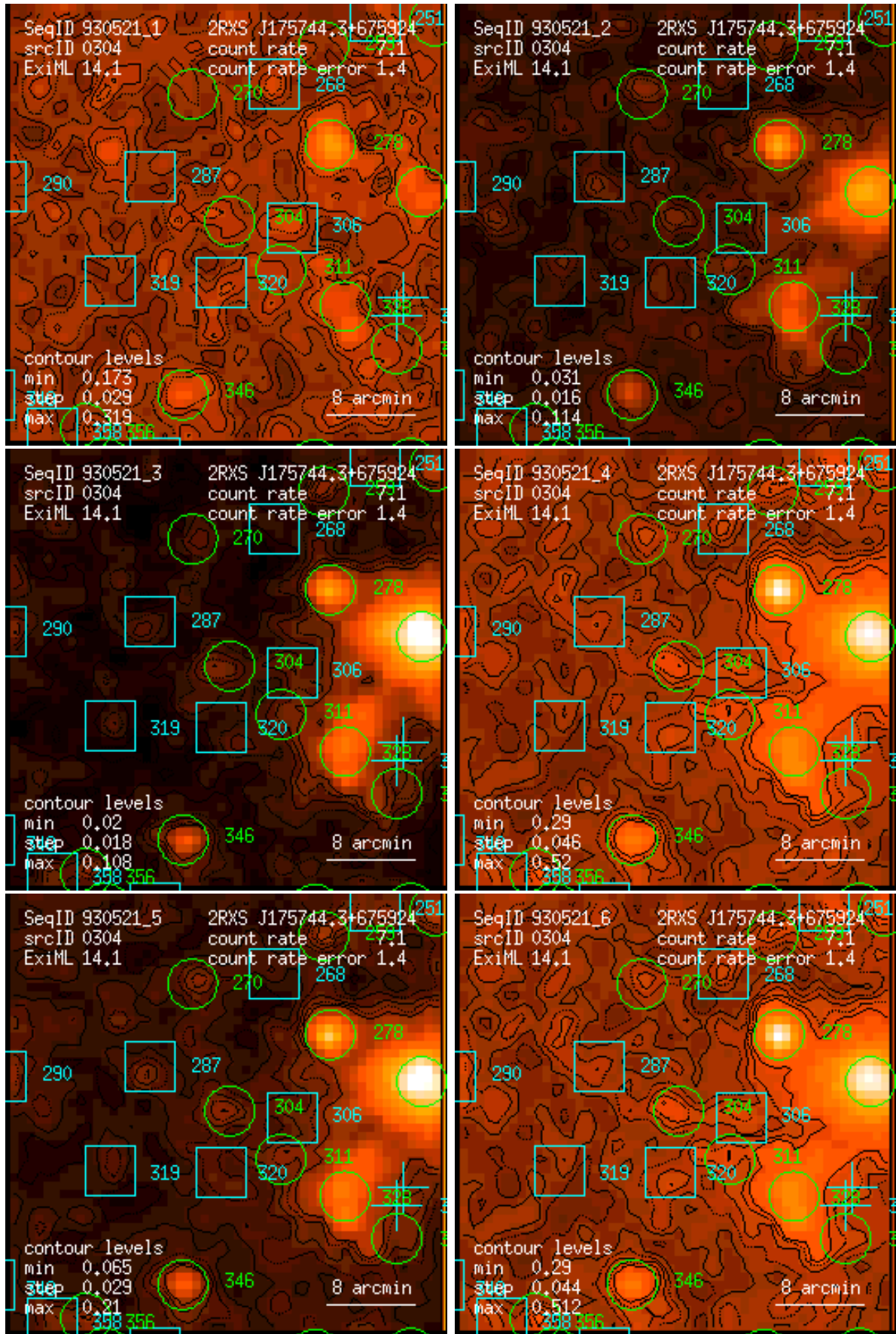
Figure 304: RASS 930521: detection 0304: band rate images, Gaussian filter: (1) PSPC channels 11 – 41, (2) 52 – 90, (3) 91 – 201, (4) 11 – 235, (5) 52 – 201, (6) 11 – 201. Broad band rates in counts/ks. Band rate contour levels in counts/ks/arcmin 2 .
