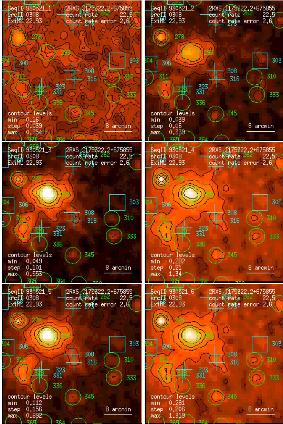
Figure 308: RASS 930521: detection 0308: band rate images, Gaussian filter: (1) PSPC channels 11 – 41, (2) 52 – 90, (3) 91 – 201, (4) 11 – 235, (5) 52 – 201, (6) 11 – 201. Broad band rates in counts/ks. Band rate contour levels in counts/ks/arcmin 2 .
