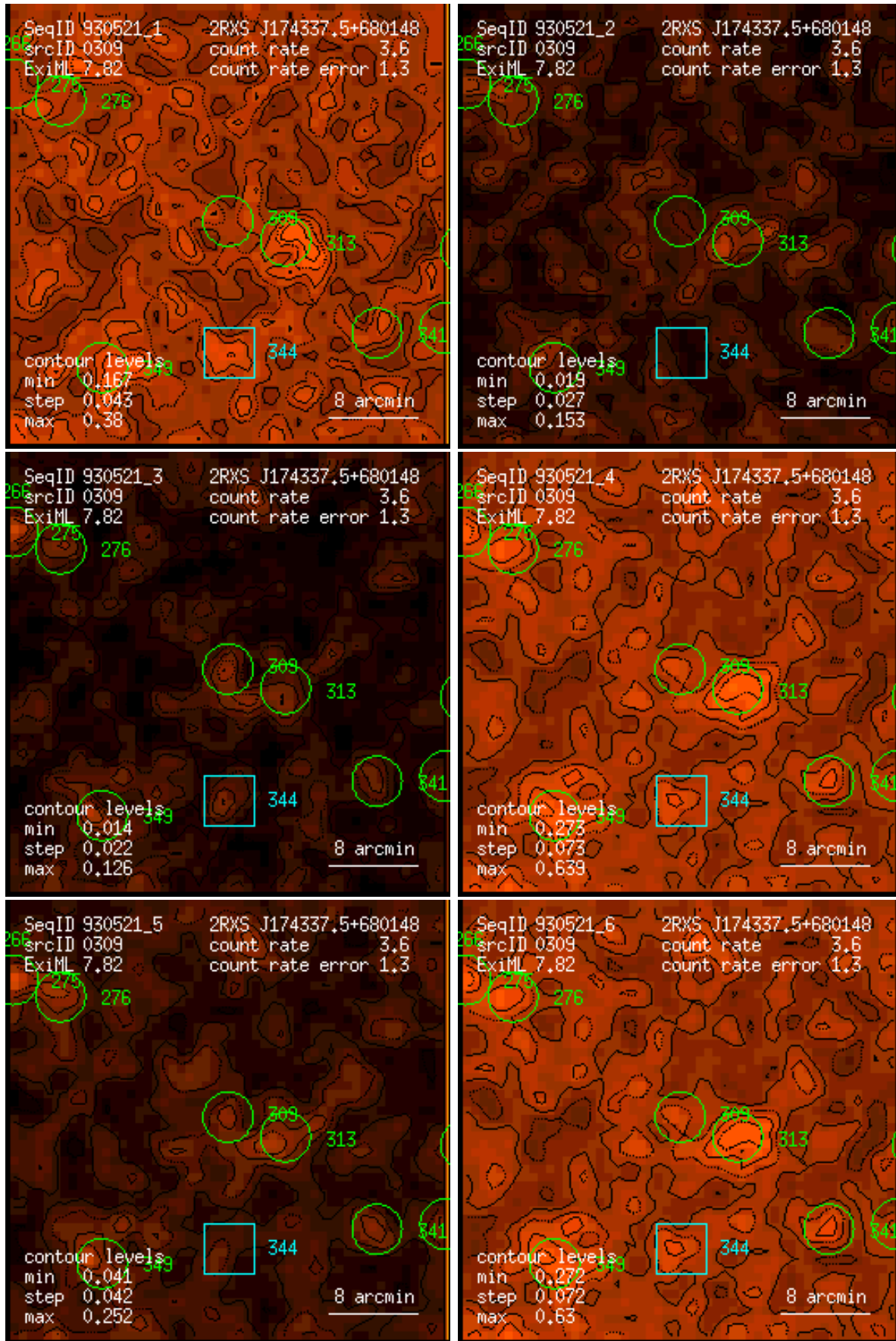
Figure 309: RASS 930521: detection 0309: band rate images, Gaussian filter: (1) PSPC channels 11 – 41, (2) 52 – 90, (3) 91 – 201, (4) 11 – 235, (5) 52 – 201, (6) 11 – 201. Broad band rates in counts/ks. Band rate contour levels in counts/ks/arcmin 2 .
