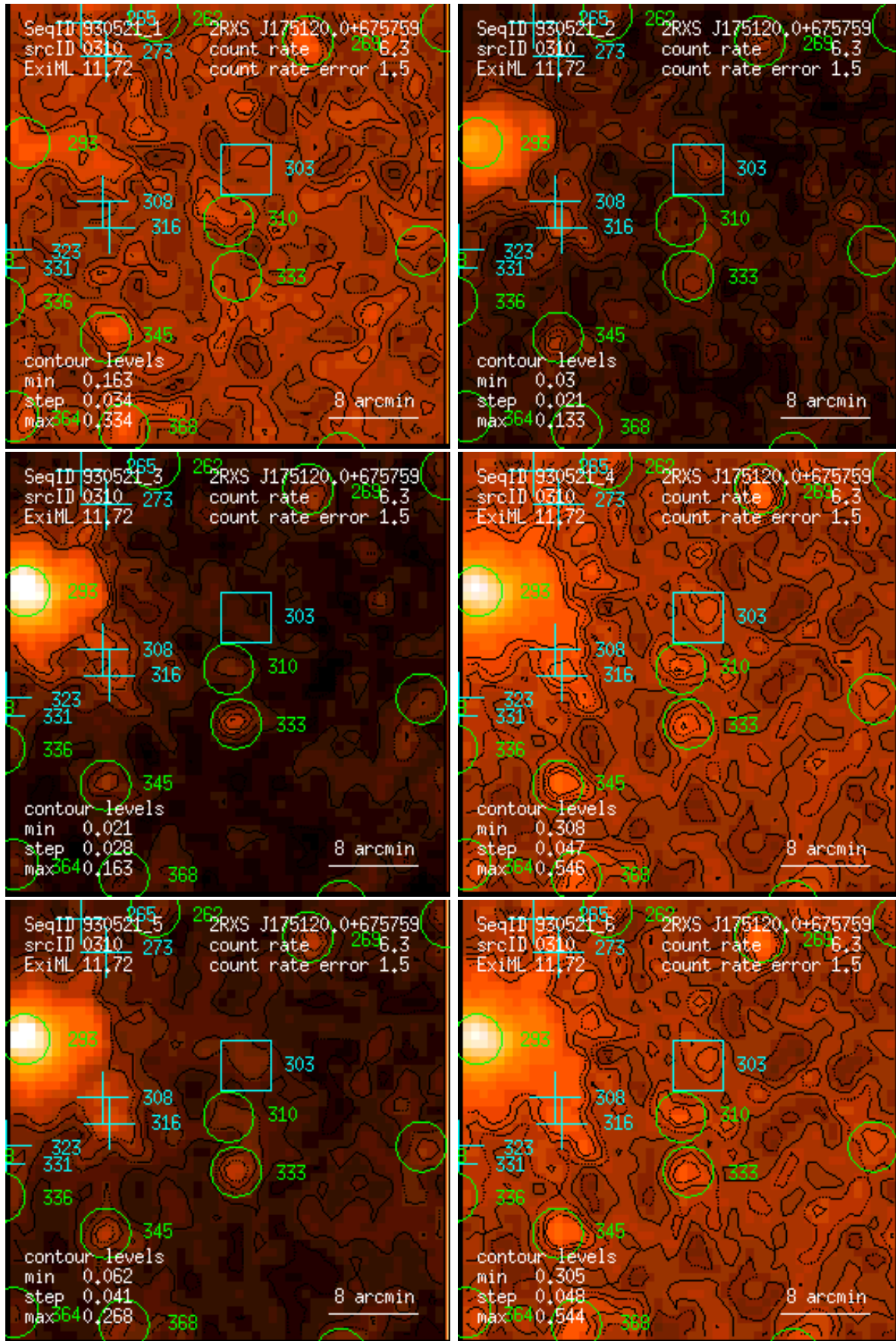
Figure 310: RASS 930521: detection 0310: band rate images, Gaussian filter: (1) PSPC channels 11 – 41, (2) 52 – 90, (3) 91 – 201, (4) 11 – 235, (5) 52 – 201, (6) 11 – 201. Broad band rates in counts/ks. Band rate contour levels in counts/ks/arcmin 2 .
