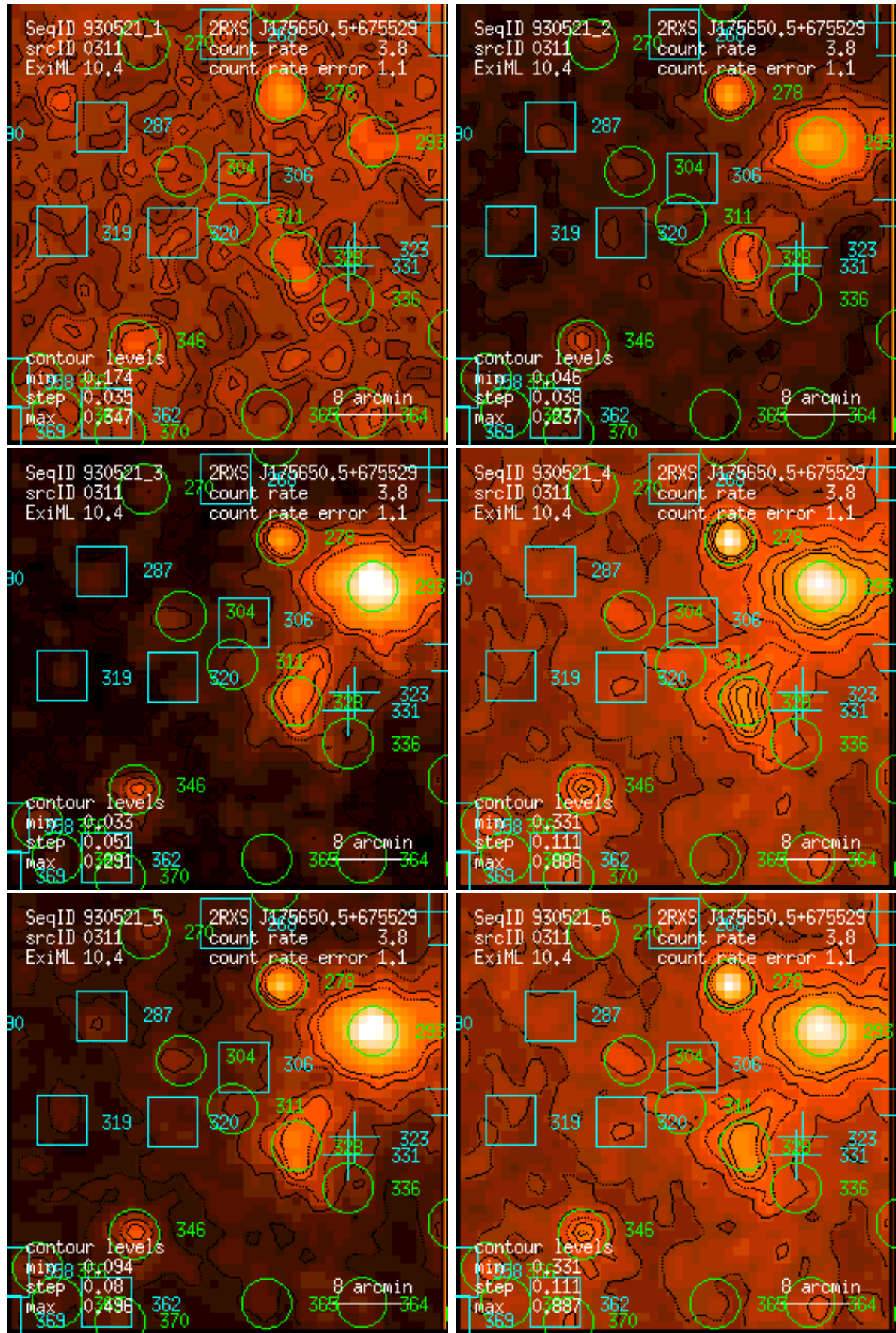
Figure 311: RASS 930521: detection 0311: band rate images, Gaussian filter: (1) PSPC channels 11 – 41, (2) 52 – 90, (3) 91 – 201, (4) 11 – 235, (5) 52 – 201, (6) 11 – 201. Broad band rates in counts/ks. Band rate contour levels in counts/ks/arcmin 2 .
