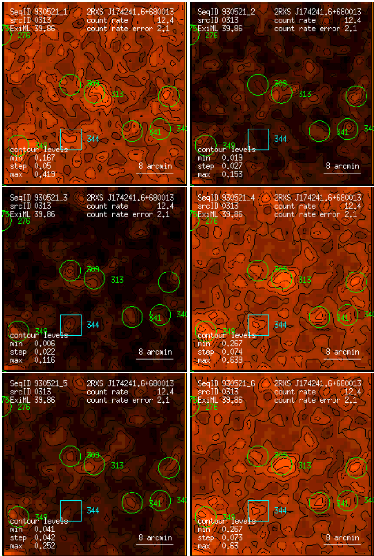
Figure 313: RASS 930521: detection 0313: band rate images, Gaussian filter: (1) PSPC channels 11 – 41, (2) 52 – 90, (3) 91 – 201, (4) 11 – 235, (5) 52 – 201, (6) 11 – 201. Broad band rates in counts/ks. Band rate contour levels in counts/ks/arcmin 2 .
